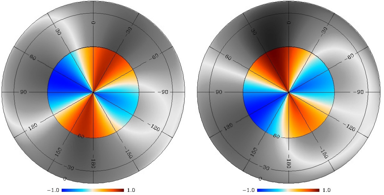
Fig. 6. Step A: orthographic projections of q_A (left) and u_A (right) centred on the south Galactic pole, for the best-fit direction of the uniform GMF towards (l_0, b_0) = (70^\circ, 24^\circ) . The sky at b > -60^\circ is masked here.
