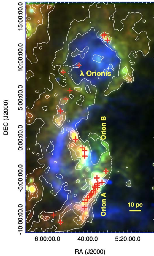
Figure 1. Spatial distribution of the observed cores (red “+”) on the three-color composite image (red: Planck 857 GHz; green: IRAS 100 \mu m; blue: H_{\alpha} ) of the Orion complex. Images are smoothed with a Gaussian kernel. White contours represent the flux density of Planck 857 GHz continuum emission. Contour levels are 14.8, 29.7, 44.5, and 59.4 MJy sr ^{-1} .
