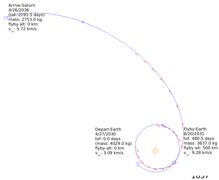
Figure 8. Interplanetary transfer to Saturn. Red arrows indicate electric propulsion thrust.
