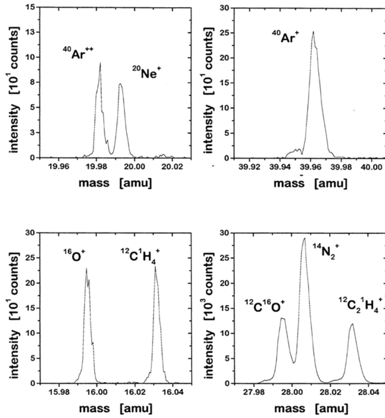
Figure 5. Separation of isobaric interference such as occur at 16, 20, 28, and 40 u/e for the indicated species is possible based on heritage of RTOF/ROSINA from the Rosetta mission (Scherer et al., 2006; Wurz et al., 2015).
