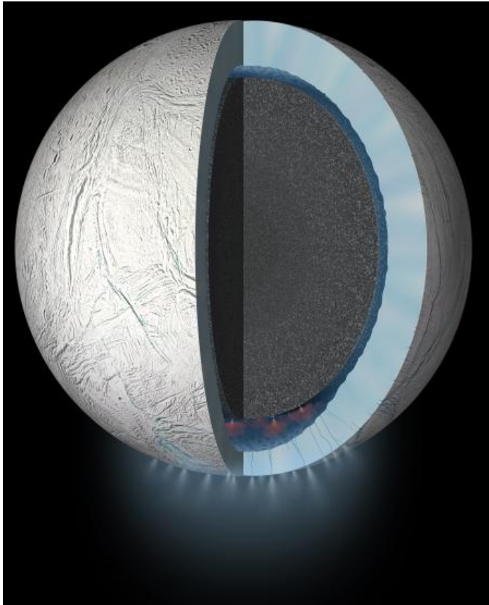
Figure 3. Enceladus' internal structure inferred from gravity, topography and libration measurement provided by Cassini mission. A global subsurface ocean is present under the outer ice shell. The ice shell is believed to be a few kilometers thin at the south polar region where the center of the geological activity is with the formation of the plume formed by multi-jets (NASA/JPL-Caltech).
