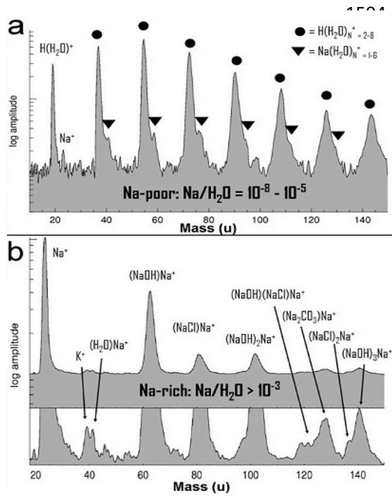
Figure 4. Composition of salt-poor (Type I and II) and salt-rich (Type III) particles in Saturn's E-ring and Enceladus' plume as measured by Cassini CDA instrument (Postberg et al., 2009).
