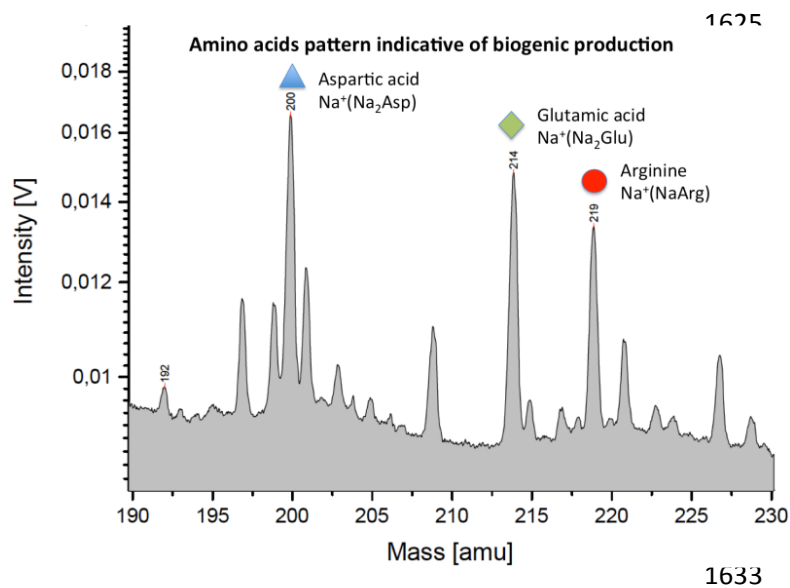
Figure 6. Laser dispersion mass spectrum of aspartic acid (12 ppm), glutamic acid (12 ppm), and arginine (8 ppm) dissolved in a salt-water matrix simulating Enceladus' ocean composition. The complex amino acids are detectable in comparable quantities to glycine (15 ppm, not shown), even though the spectrum has a mass resolution 3 times less than ENIJA's. S/N ratio of this laser dispersion spectrum is comparable to a much lower analysed concentration in ENIJA spectra ( \leq 1 ppm). Most un-annotated mass lines are due to salt-water cluster ions. By co-adding multiple ice grain spectra the S/N ratio can be further improved leading to an ENIJA detection limit of 10–100 ppb for most amino acids in ice grains formed from Enceladus' ocean water.
