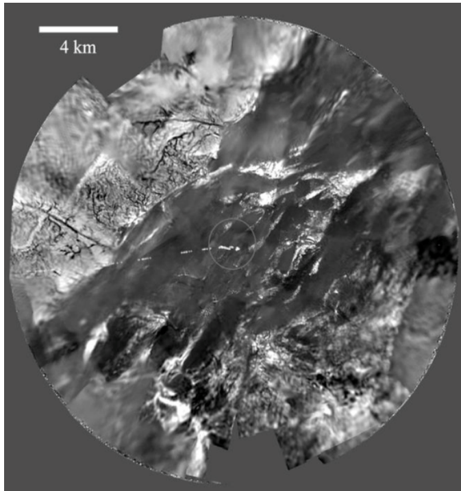
Figure 7. The surface of Titan imaged by DISR camera during the Huygens probe descend. TIGER has the capability to image Titan at Huygens DISR resolution (ESA/NASA/JPL/University of Arizona).
