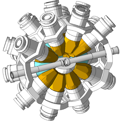
FIG. 1. One hemisphere of the TAC showing the \text{BaF}_2 crystals and photomultipliers mounted in the support structure. The vacuum time-of-flight tube traversing the detector is split at the center of the TAC where the sample holder in air is positioned, surrounded by the neutron absorber of which only the lower half is shown.
