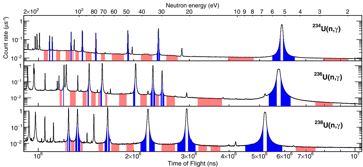
FIG. 2. The time-of-flight spectra for the (n, \gamma) reactions on ^{234}\text{U} , ^{236}\text{U} , and ^{238}\text{U} for m \geq 2 TAC events. The top axis shows the corresponding neutron-energy scale. The blue regions are used for the analysis while the red ones correspond to the windows for the background subtraction; see text for details.
