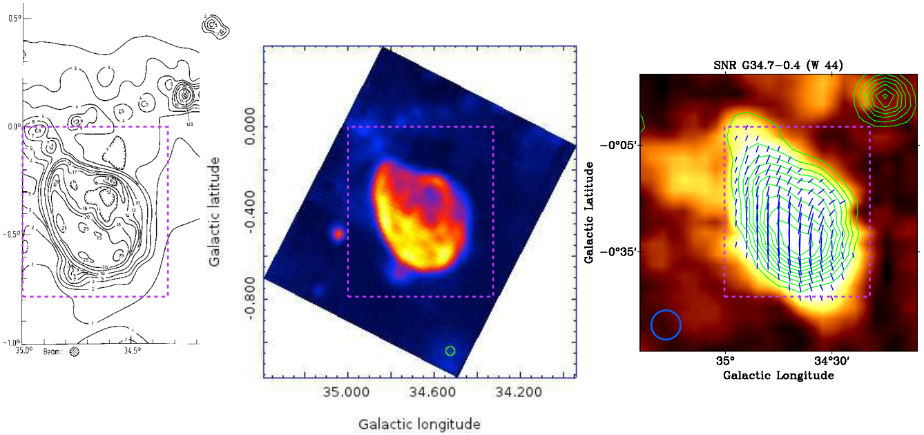
Figure 7. Left: contour map obtained by Effelsberg at 4.9 GHz (Altenhoff et al. 1979), middle: SRT observation at 7 GHz, right: intensity contours (indicated in green) obtained with Urumqi at 4.8 GHz (Sun et al. 2011). The dotted rectangles indicate the same sky region. The blue and green circles in the bottom corner of the maps show the beam size.
