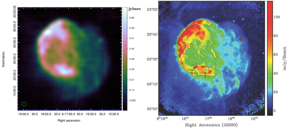
Figure 6. Comparison of the continuum maps of IC443 obtained with SRT at 7 GHz (left) with that obtained combining VLA and Arecibo at 1.4 GHz (Lee et al. 2008).
