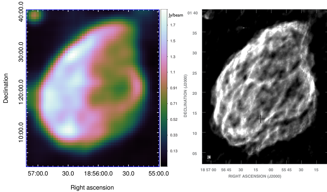
Figure 8. Comparison of the continuum maps of SNR W44 obtained with SRT at 7.0 GHz (left) with that obtained with the VLA at 324 MHz (right) (Castelletti et al. 2007). The beam size in the SRT map is represented by the point-like source in the top left corner.
