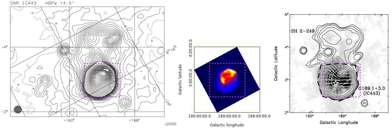
Figure 5. Comparison of the radio continuum emission of SNR IC443 as seen with different single-dish telescopes. Left: Contour plot observed at 868 MHz with Effelsberg (Reich et al. 2003). Middle: SRT observation at 7.2 GHz in Galactic coordinates. Right: Radio continuum and polarization image of IC443 obtained with Urumqi at 5 GHz (Gao et al. 2011). The dotted rectangles indicate the same sky region.
