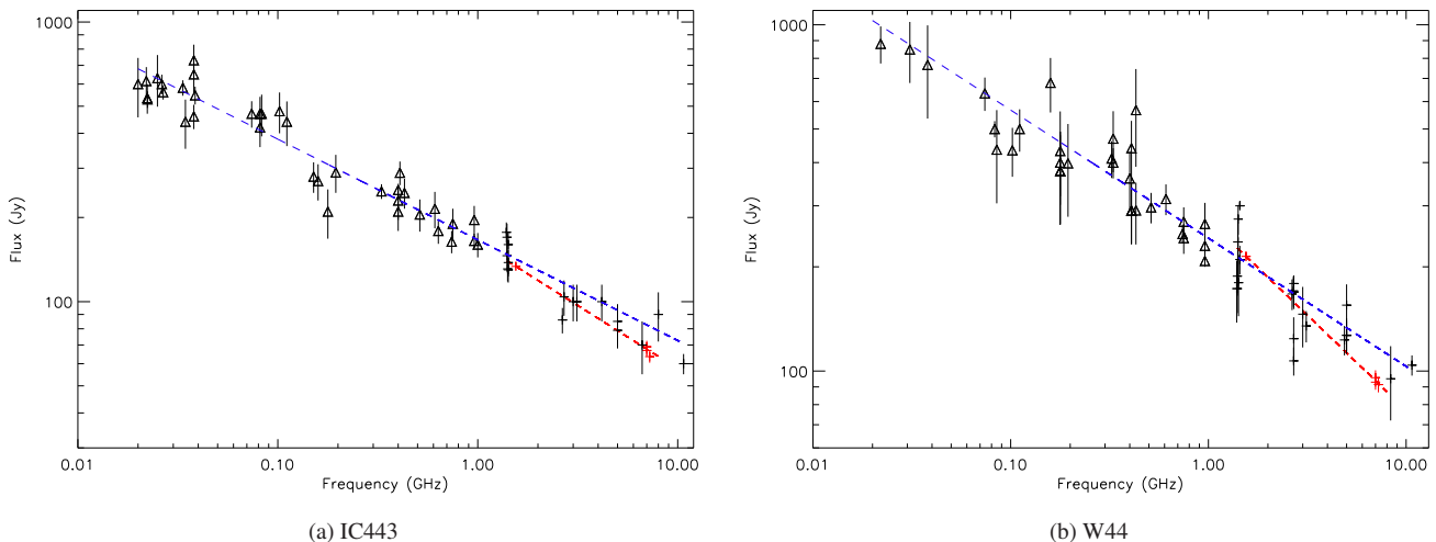
Figure 9. Integrated radio continuum spectra of IC443 (a) and W44 (b) obtained from the flux density values (black points) listed in Castelletti et al. (2011, 2007) for the frequency range 0.02 – 10.7 GHz together with the fit provided by these authors (blue dashed line). The spectral slopes derived from SRT data (Tables 2 and 3; red points and dashed line) at high frequencies (1.5 – 7.2 GHz) suggest a possible spectral steepening with respect to the lower frequency measurements (0.02 – 1 GHz; triangles).
