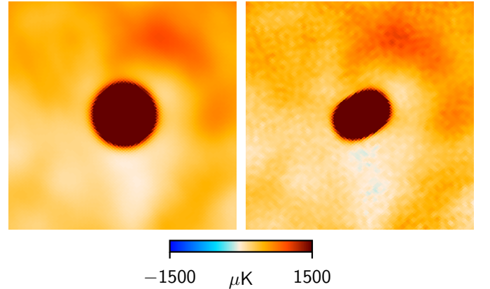
Fig. 2. A 10^\circ patch around the Crab Nebula in the 30-GHz temperature map. Left: deconvolved. Right: PR3 30-GHz LFI map.
