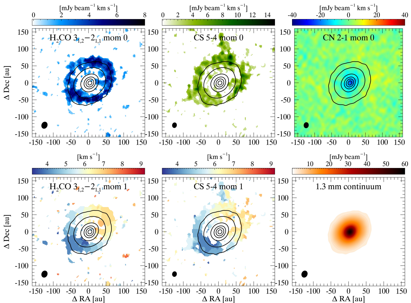
Fig. 1. Moment-0 maps (top panels) of \text{H}_2\text{CO} 3_{1,2} - 2_{1,1} (left), CS 5 - 4 (middle), and CN 2 - 1 (right; blending of the three components at 226.87 GHz reported in Table 1) towards DG Tau. The corresponding moment-1 maps are shown in the bottom left and middle panels, while no moment-1 map is shown for CN 2 - 1 because of the blending of the three hyperfine components. The bottom right panel shows the map of the continuum emission at 1.3 mm. The color scale indicates the line intensity in \text{mJy beam}^{-1} \text{km s}^{-1} (moment-0), the velocity V_{\text{LSR}} in \text{km s}^{-1} (moment-1), and the intensity in \text{mJy beam}^{-1} (for the continuum map). The black contours indicate the 1.3 mm dust continuum emission (0.01% corresponding to the 5\sigma level, 10%, 30%, 50%, 70%, and 90% contours). The ellipse in the bottom left corner of each panel shows the ALMA synthesized beam.
