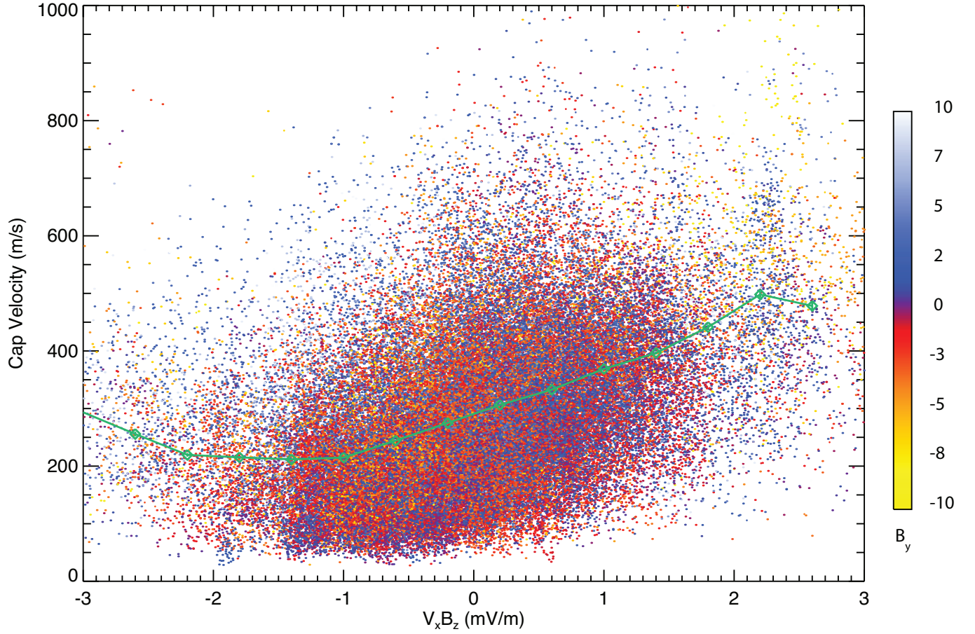
Figure 7. Scatter plot showing the observed velocity in the polar cap versus the product of the radial component of the solar wind velocity with the z-component of the IMF. Each point is an average of all measurements within the 85° latitude circle.
