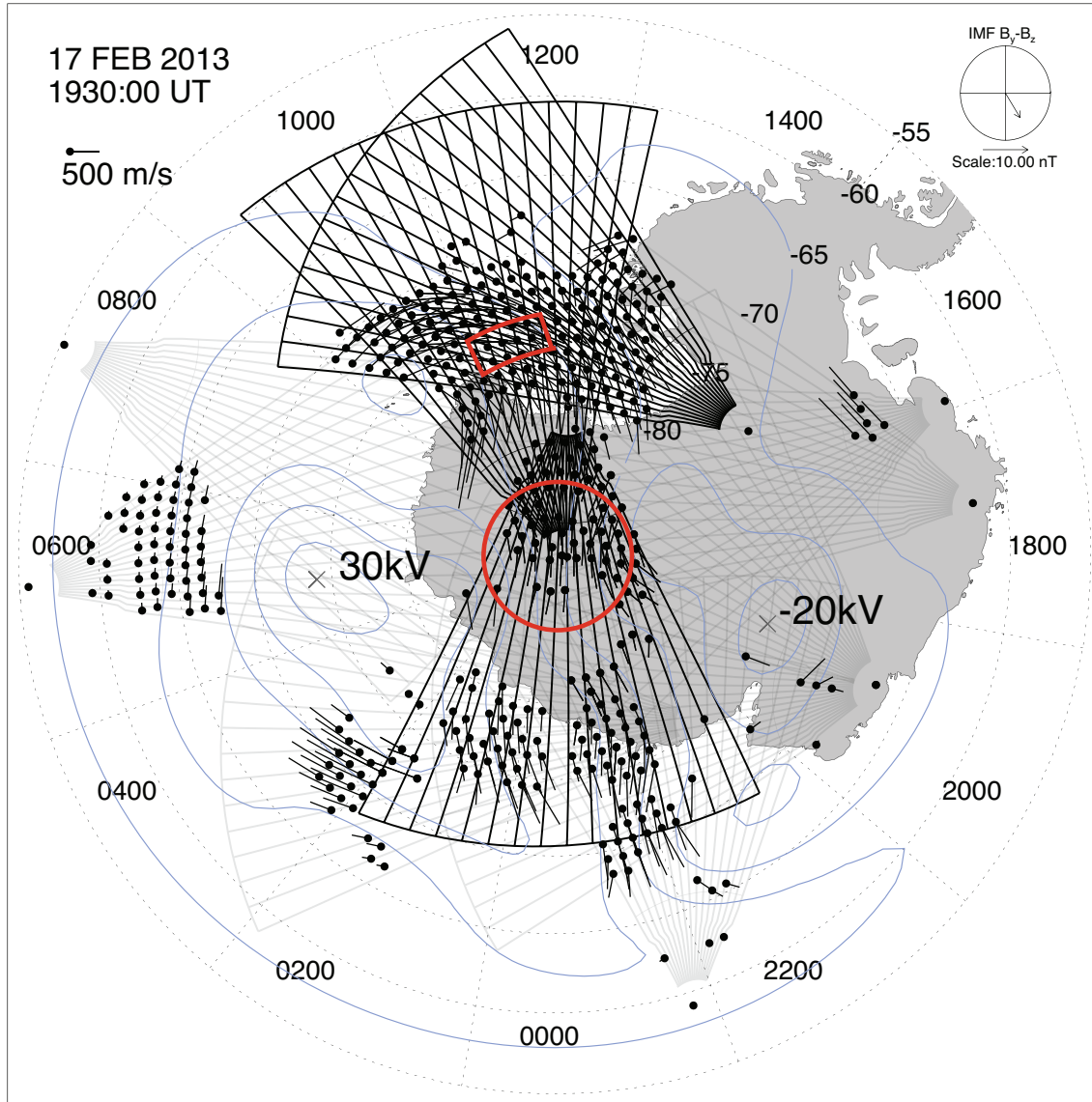
Figure 3. Convection map for 1930 UT on February 17, 2013. Fields of view of the McMurdo, South Pole, and Dome C radars are superposed. The red circle at 85° indicates the area defined as the central polar cap. The red box indicates the area defined as the dayside throat.
