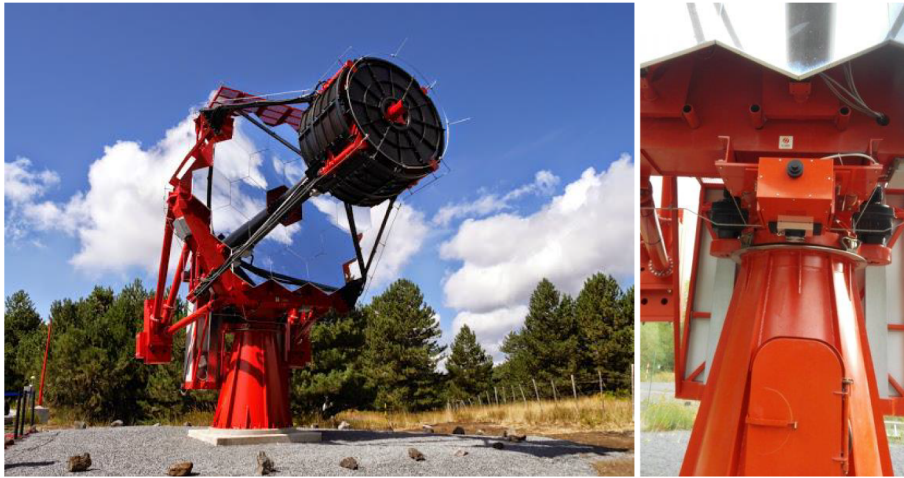
Fig. 1 ASTRI-Horn, the dual-mirror Cherenkov telescope installed on Mt.Etna, Italy, at the INAF “M.C. Fracastoro” observing station. On the right panel it is visible the small UVscope instrument mounted under the primary mirror structure of the ASTRI-Horn telescope
