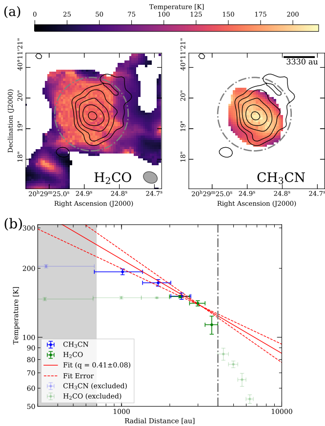
Fig. 4. (a) H 2 CO and CH 3 CN temperature maps derived with XCLASS at a threshold of 10\sigma . The black contours show the 1.37 mm continuum emission with levels at 5, 10, 20, 40, and 80\sigma ( \sigma = 0.59 mJy beam -1 ). The gray dash-dotted circle indicates the outer radius of the radial temperature fit (bottom panel). The beam size ( 0.''47 \times 0.''36 ) is shown in the lower right corner of the H 2 CO temperature map. (b) Radial temperature profiles obtained from the data in the top panel. The data are binned in steps of half a beam size ( \sim 700 au) for H 2 CO (green data points) and CH 3 CN (blue data points). A power-law fit was performed on spatial scales in the range 700 – 4000 au to determine the temperature power-law index q . The gray dash-dotted line indicates the outer radius of the radial temperature fit. At radii smaller than 700 au the temperature profile cannot be determined due to the finite beam size (gray shaded area). The transparent data points were excluded from the fitting. The best fit is shown by the red solid line. The error of the fit (one standard deviation) is shown by the red dashed lines.
