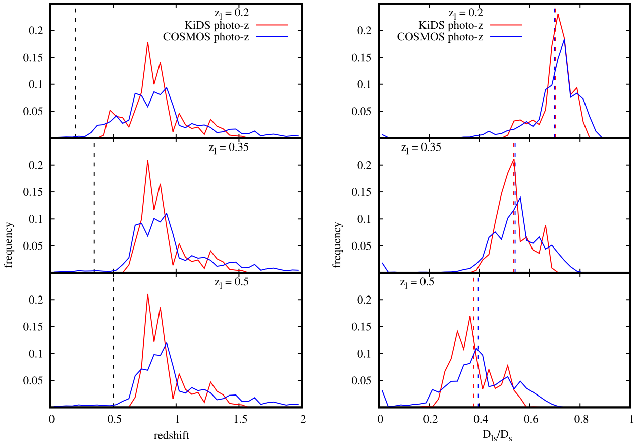
Figure 6. Left: Redshift distributions of the background sample, as estimated from photo-zs by KiDS (red line) and COSMOS (blue line). The black dashed line represents the assumed cluster redshift, i.e. 0.2, 0.35, and 0.5 for the top, middle, and bottom panel, respectively. Right: Distribution of D_{ls}/D_s for the background sample, as estimated from KiDS photometric redshifts (red line) and COSMOS ones (blue line). The dashed lines represent the mean D_{ls}/D_s for the sample. The top, middle, and bottom panels refer to different cluster redshifts, with z_l = 0.2, 0.35 , and 0.5 , respectively.
