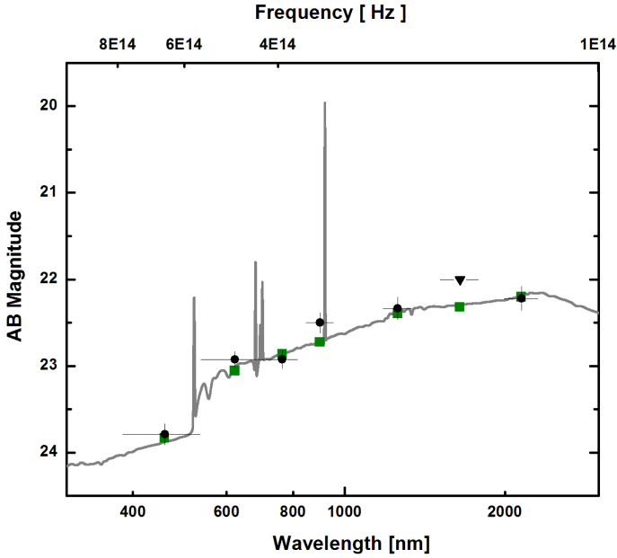
Fig. A.6. SED of the host galaxy of GRB 120714B based on GROND g'r'i'z' and HAWKI JK_s -band data. The SED is best described by a galaxy undergoing an episode of intense star-forming activity (for the color coding see Fig. A.2).
