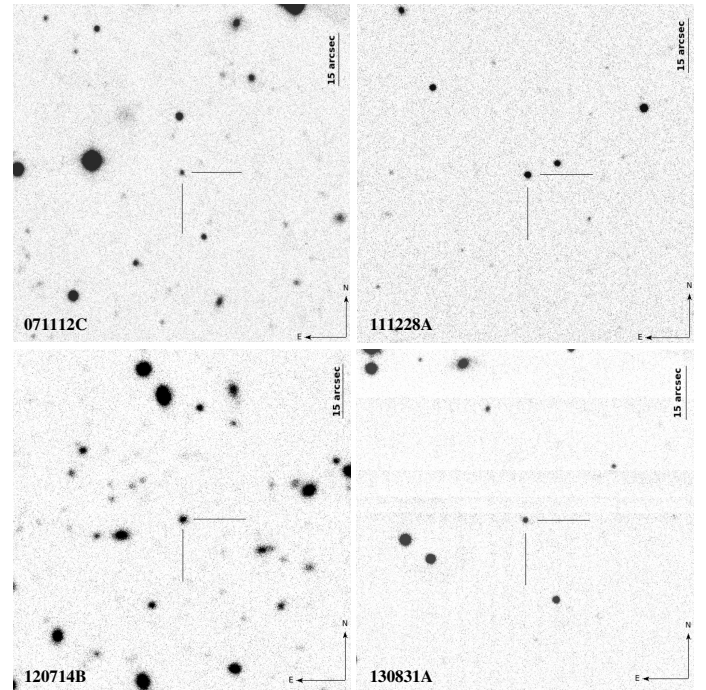
Fig. A.9. Finding charts of the GRB fields. Shown here are the afterglows as imaged by GROND in the r' band. Top left panel: 0.369 days after the burst, top right panel: 0.648 days, bottom left panel: 0.396 days, bottom right panel: 0.689 days.
