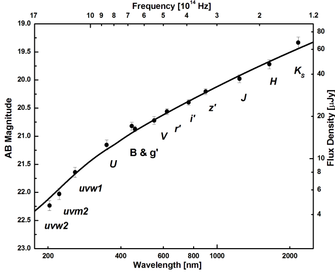
Fig. A.4. SED of the afterglow of GRB 111228A based on GROND as well as Swift /UVOT data (Tables C.7, C.8). Magnitudes refer to the time of the light curve break at t = t_b = 1 day, i.e., are free of any contribution from an underlying SN component. Data are corrected for Galactic extinction. The SED suggests a host extinction of A_V^{\text{host}} = 0.16 mag.
