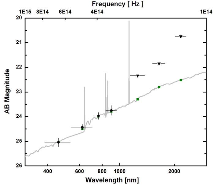
Fig. A.5. SED of the host galaxy of GRB 111228A based on GROND data taken four years after the burst and the corresponding best galaxy-template SED found by Le PHARE (for the color coding see Fig. A.2). Due to the lack of a NIR detection, the fit is rather ill-defined.
