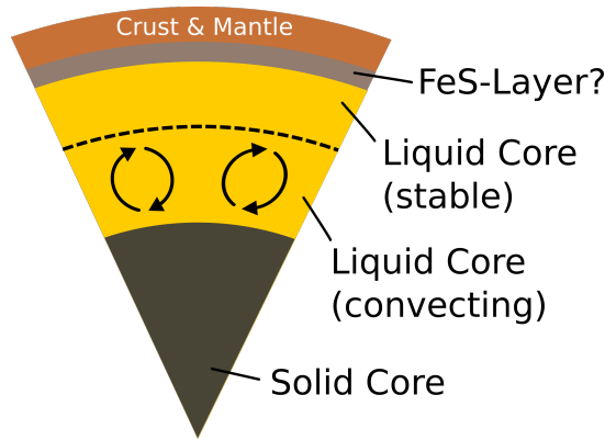
Fig. 11 Possible interior structure of Mercury with a stably stratified liquid core layer.
