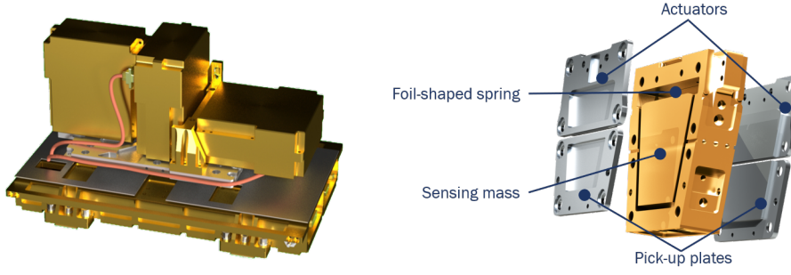
Fig. 2 (left) Configuration of ISA sensors, and (right) naked accelerometer and foil-shaped spring (Images courtesy of Thales Alenia Space).
