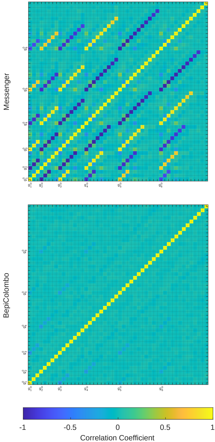
Fig. 7 Correlation matrices of the internal Gauss coefficients retrieved after the MESSENGER mission ( top ) and through the numerical simulations of the BepiColombo mission ( bottom ). The order of the coefficients is: g_1^0, g_1^1, h_1^1, g_2^0, g_2^1, \dots . Terms with m \neq 0 are not shown for readability reasons.
