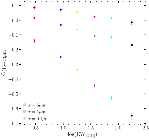
Figure 3. Energy slopes, as defined in Eq. 1, for the six stacked representative SED. Circles, squares and diamonds indicate the slope (15-6)\mu\text{m} , (15-1)\mu\text{m} and (15-0.1)\mu\text{m} respectively.
