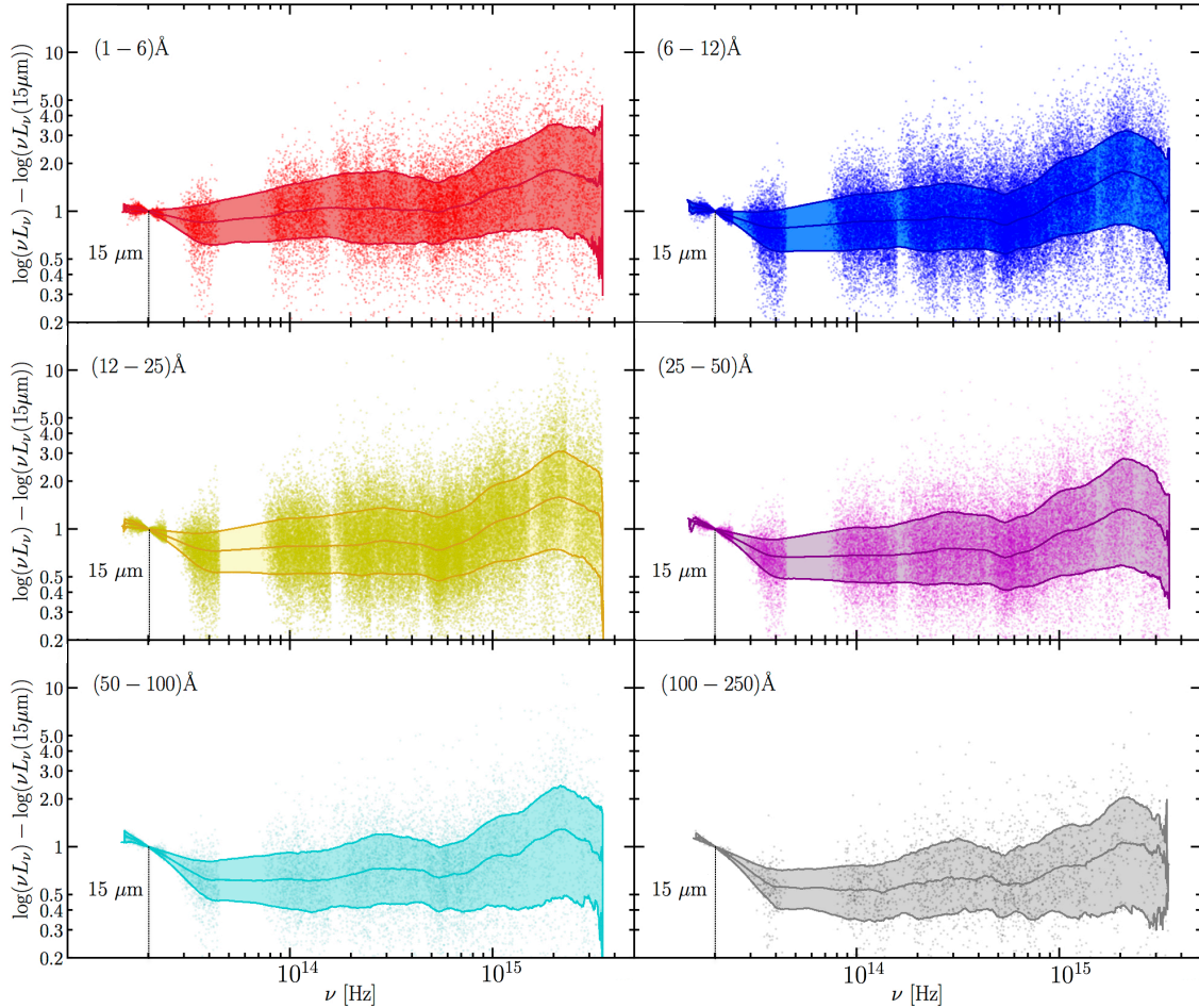
Figure 1. Rest-framed photometric data points for each source in the sample (points) in six EW[O III] intervals, normalised to the flux corresponding to the reference wavelength \lambda = 15\mu\text{m} . The solid lines are the 84 th , 50 th (median) and 16 th percentiles - in each spectral channel - of the distribution of the SED obtained by interpolating the photometric data points for each source.
