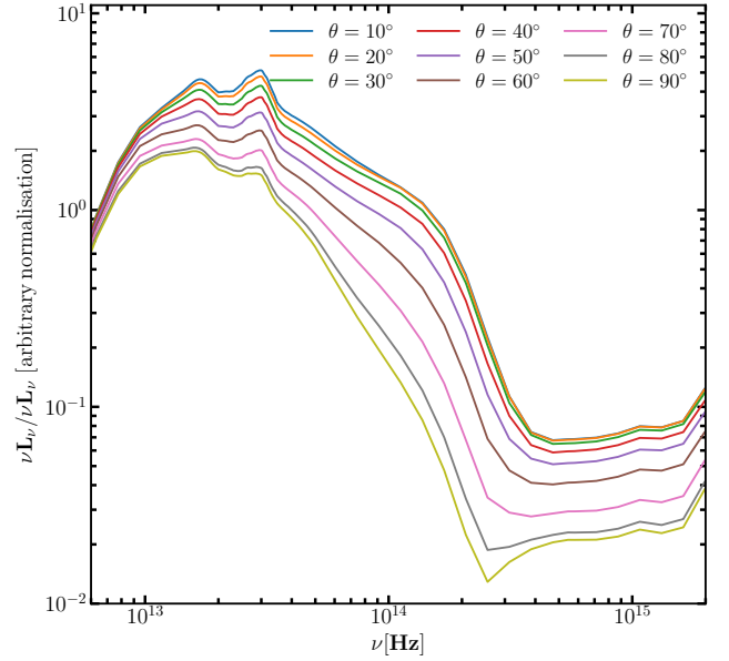
Figure 4. CLUMPY models as a function of the inclination angle of the torus with respect to the line of sight. The CLUMPY library contains more than 10^6 theoretical SED, obtained varying the set of parameters describing the physics and geometry of the torus.
