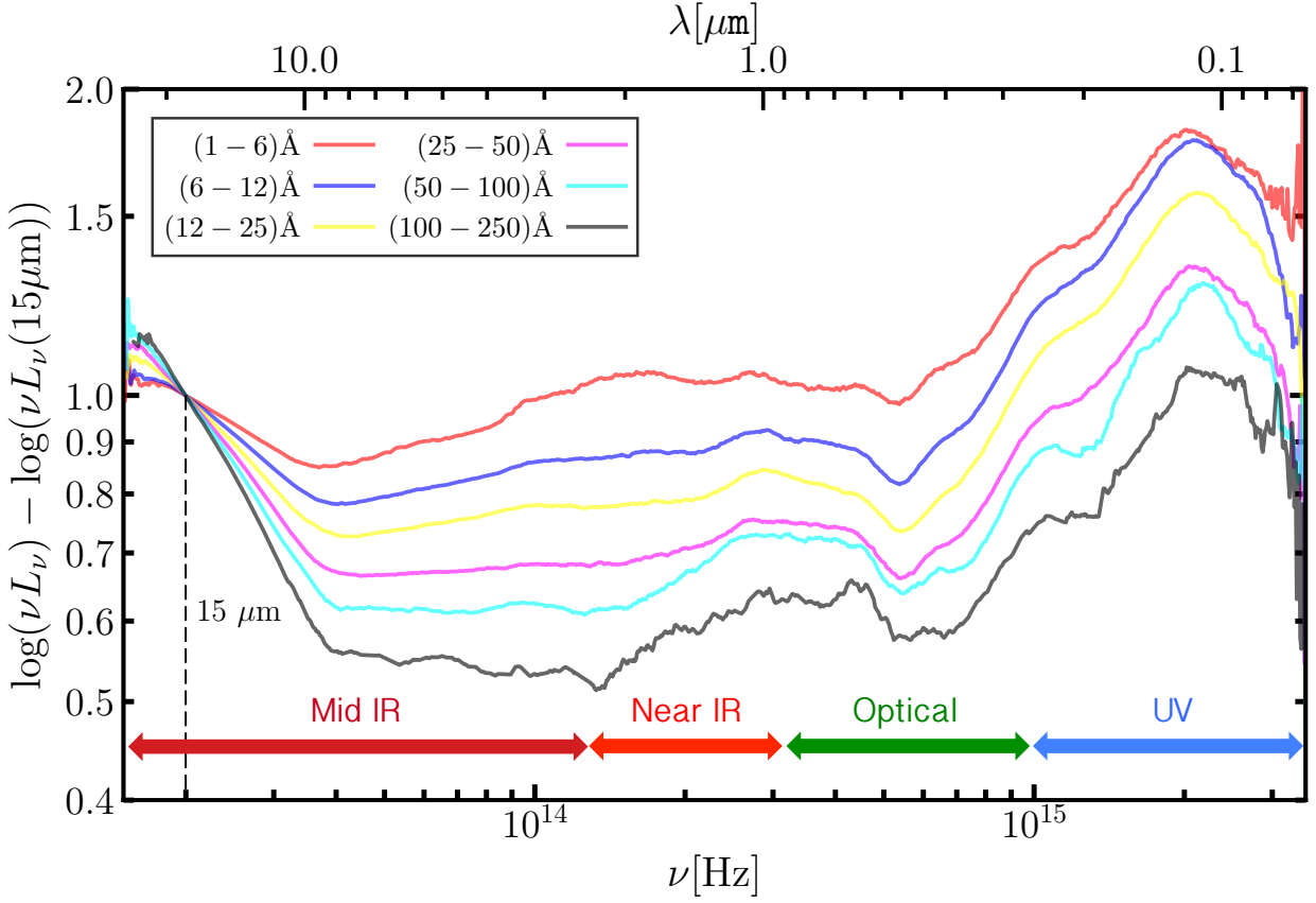
Figure 2. Comparison of the stacked SED obtained from the photometric data points for the six EW[O III] bins. Moving to high EW[O III], we see the IR part of the SED steepening, as expected in a clumpy torus scenario.
