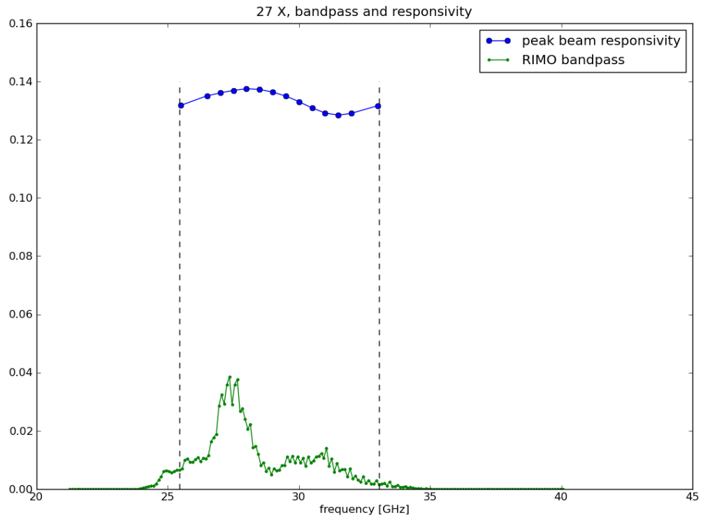
Figure 2: The normalized bandpass for 27 X from RIMO (green points) and the peak beam responsivity (blue points) D_\nu(\hat{\mathbf{0}}) , arbitrarily scaled to fit the plot. The black lines mark the frequency interval taken in consideration.
