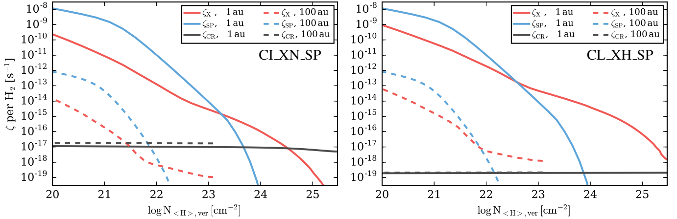
Fig. 6. Ionization rates \zeta as a function of vertical column density N_{(H),\text{ver}} at radii of 1 and 100 au (solid and dashed lines respectively). The maximum values for N_{(H),\text{ver}} at the midplane of the disk, are N_{(H),\text{ver}} \approx 4 \times 10^{25} \text{ cm}^{-2} and N_{(H),\text{ver}} \approx 2 \times 10^{23} \text{ cm}^{-2} at 1 au and 100 au, respectively. Red lines are for X-rays, blue lines are for SPs and the black lines are for CRs. Left panel: model CL_XN_SP with ISM CRs and normal X-rays; right panel: model CL_XH_SP with low CRs and high X-rays.
