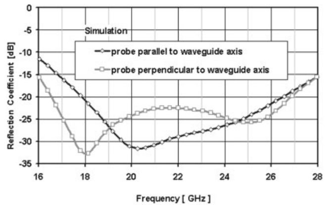
Figure 2 Simulated reflection coefficient at the 50- \Omega microstrip chip port for probe orientation parallel (longitudinal probe, rhomb dotted line) and perpendicular (broadside probe, square dotted line) to the waveguide axis
