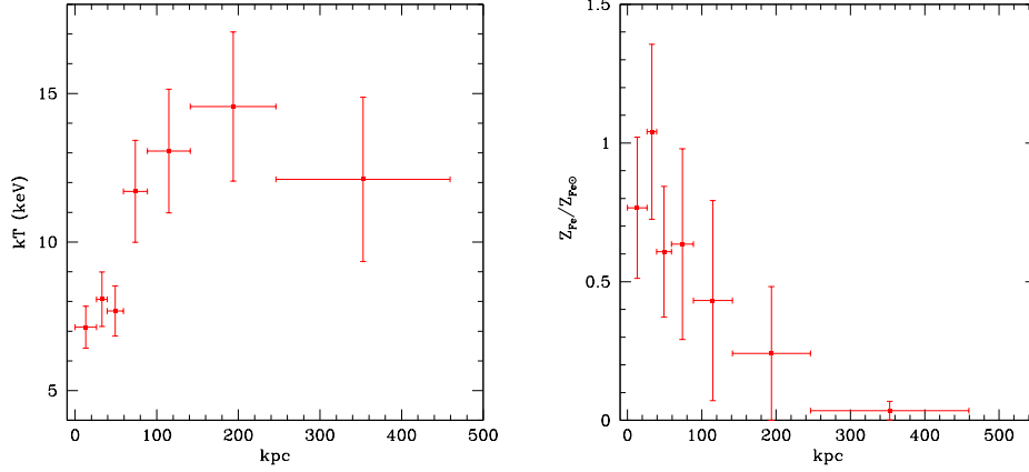
Fig. 1. Left panel: projected temperature profile of SPT-CLJ2344 obtained from the 11.7 ks Chandra ACIS-I observation, after removing the central AGN. Errorbars correspond to 1\sigma . Right panel: projected iron abundance profile of SPT-CLJ2344 from Chandra data.
