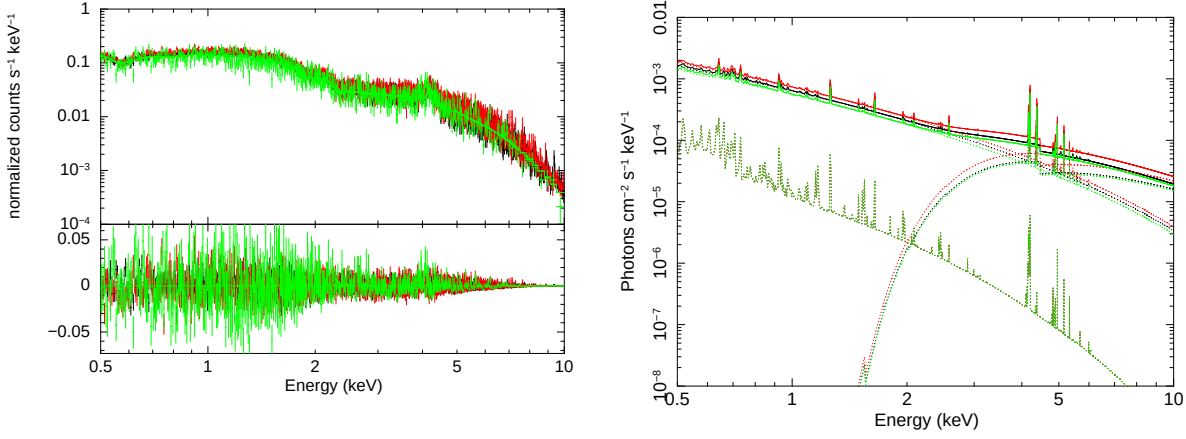
Fig. 3. Left panel: MOS spectra from the three Obsids with best-fit model obtained for a single mckflow in the 0.3–3.0 keV temperature range. The lower panel shows the residual with respect to the best-fit model. Right panel: components of the best-fit model of the MOS spectra (three for each component, shown with dotted lines) obtained for a single mckflow in the 0.3–3.0 keV temperature range. The mckflow component is the lower thermal component, while the AGN contribution is virtually negligible below 2 keV.
