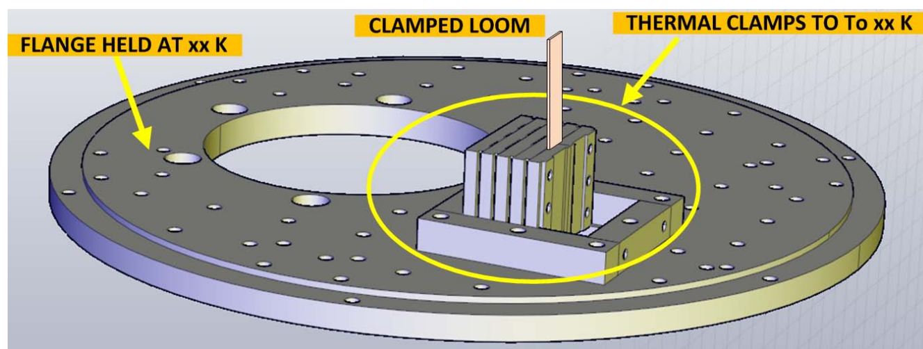
Fig. 5.5.4.1: example of the envisaged thermal clamp
