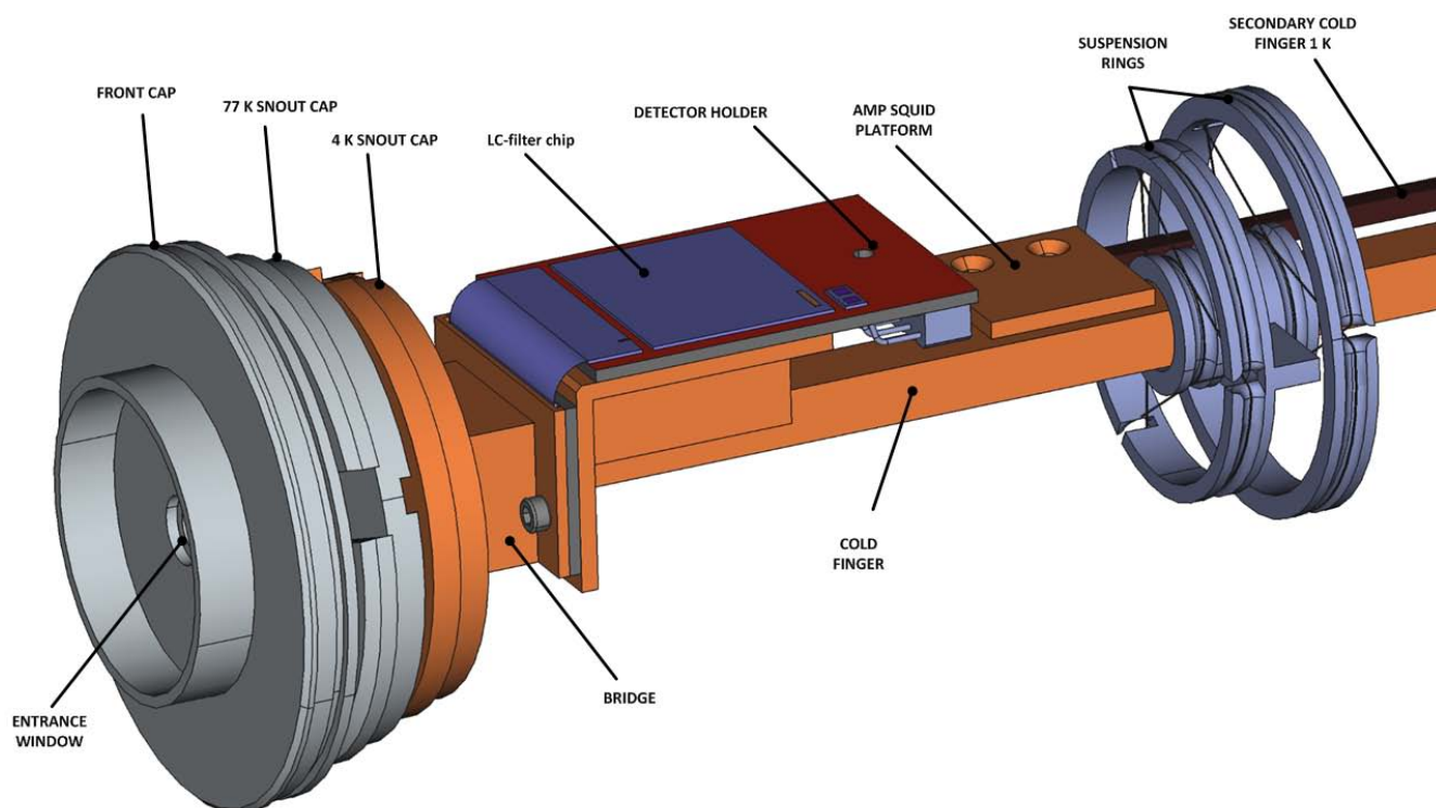
Fig. 5.1.4.1: rendering of the main components of the snout with nomenclature
