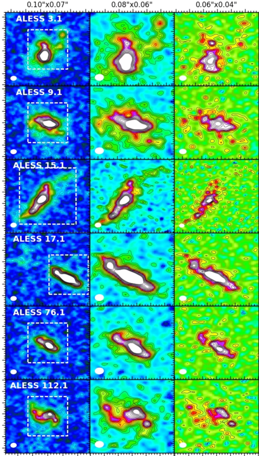
Figure 1. ALMA maps of the 770 \mu\text{m} continuum emission from six SMGs imaged at three different resolutions (indicated above each column). Contours start at \pm 2\sigma and go in steps of 1\sigma , stopping at 30\sigma (left), 20\sigma (middle), and 10\sigma (right) for clarity. These images reveal resolved structure on scales of \sim 0.07'' ( \sim 500 pc at z \sim 2.5 ), with large-scale structures suggestive of spiral arms and bars. Left column: 1.3'' \times 1.3'' maps imaged with natural weighting, resulting in an rms of \sigma \sim 20 \mu\text{Jy beam}^{-1} and a resolution of 0.10'' \times 0.07'' . The dashed white box indicates the region shown in the two right columns and is 0.7'' \times 0.7'' for all sources except ALESS 15.1, where a larger 1.0'' \times 1.0'' region is shown. Middle column: zoomed-in maps of the region indicated in the left column, now imaged with Briggs weighting ( R = +0.5 ), resulting in an rms of \sigma \sim 22 \mu\text{Jy beam}^{-1} and a resolution of 0.08'' \times 0.06'' . Right column: zoomed-in maps of the region indicated in the left column, now imaged with a different Briggs weighting ( R = -0.5 ), resulting in an rms of \sigma \sim 42 \mu\text{Jy beam}^{-1} and a resolution of 0.06'' \times 0.04'' .
