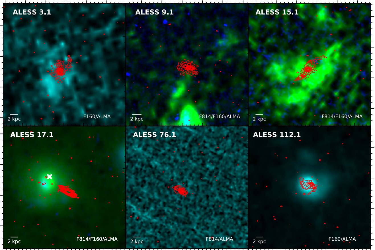
Figure 2. 4'' \times 4'' false-color images of the HST and ALMA data for each of our sources. Shown are the HST H_{160} band (green), the HST I_{814} band (blue), and the ALMA 870\ \mu\text{m} emission at 0''.08 \times 0''.06 resolution (middle column of Figure 1; red contours). The position of the X-ray source in ALESS 17.1 is indicated by the white cross. ALMA contours are shown at 3\sigma , 6\sigma , 9\sigma , 12\sigma , ..., and the HST stretch has been adjusted to enhance the visibility of faint emission as needed. This comparison suggests that the ALMA imaging may be revealing the starbursting cores of more extended highly obscured systems.
