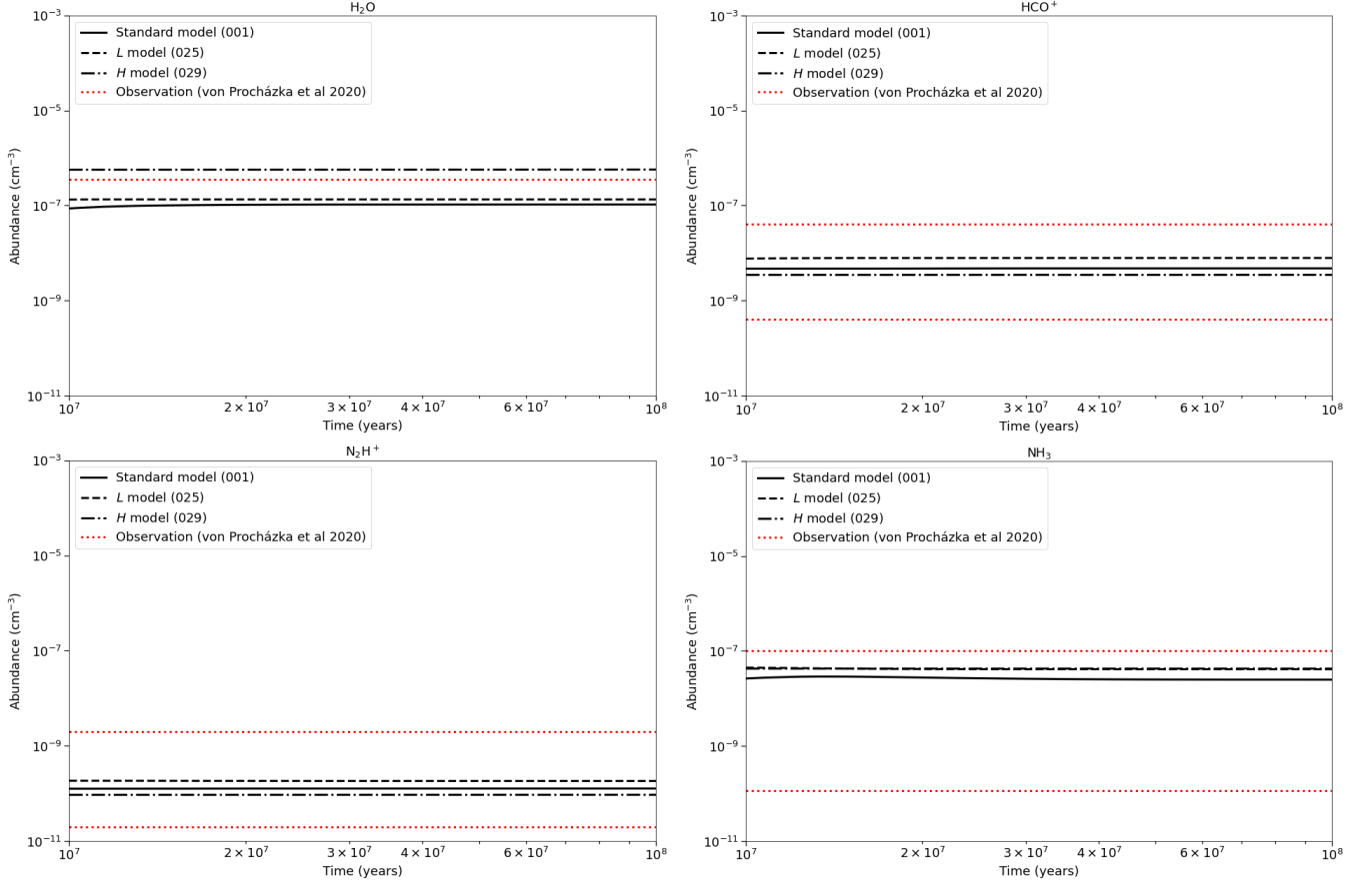
Figure 7. Figure showing the upper and lower limits to species in TMC-1, derived from von Procházka & Millar (2020). Figures compare observed abundances of \text{H}_2\text{O} (top left), \text{HCO}^+ (top right), \text{N}_2\text{H}^+ (bottom left) and \text{NH}_3 (bottom right) limits to UCLCHEM post-collapse models. The red dotted lines show the upper and lower limits (for \text{H}_2\text{O} there are only upper limits).
