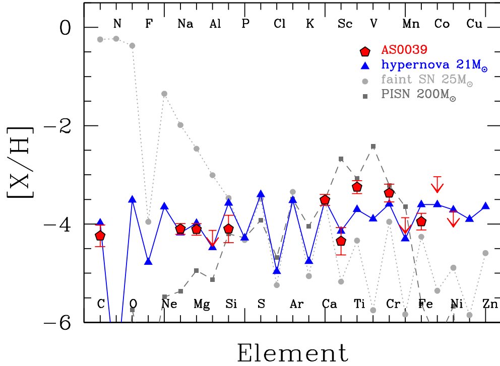
Figure 3. The NLTE abundance pattern of AS0039 (red pentagons) compared to theoretical models. Blue triangles show the best fitting model of a zero-metallicity 21 M_{\odot} hypernovae, of energy 10 \times 10^{51} erg. Also depicted are models for a PopIII faint supernova of 25 M_{\odot} with E = 0.7 \times 10^{51} erg (light grey circles), and pair instability supernova of 200 M_{\odot} (dark grey squares). All models are normalized to the measured [Ca/H]_{NLTE} of AS0039. The C abundance of AS0039 has been corrected for internal mixing (Placco et al. 2014).
