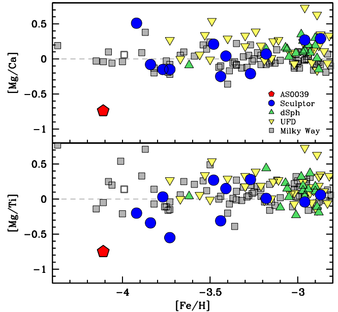
Figure 2. Comparison of the 1D LTE \alpha -element ratios of AS0039 to those of the literature, [\text{Mg}/\text{Ca}] (top) and [\text{Mg}/\text{Ti}] (bottom). Classical 1D LTE abundances for RGB stars in Sculptor (blue), other dSph galaxies (green), the UFD galaxies (yellow), and C-normal RGB stars in the Milky Way (Suda et al. 2008). The Milky Way star SPLUS J210428.01-004934.2 (Placco et al. 2021) is shown with a gray open square.
