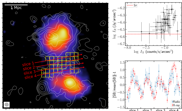
Figure 4. Chandra smoothed image in the 0.5 – 2.0 keV band overlaid with the low-resolution LOFAR HBA contours ( left ). The boxes and slices indicate the regions where the X-ray and radio surface brightness have been evaluated and compared ( right ).
