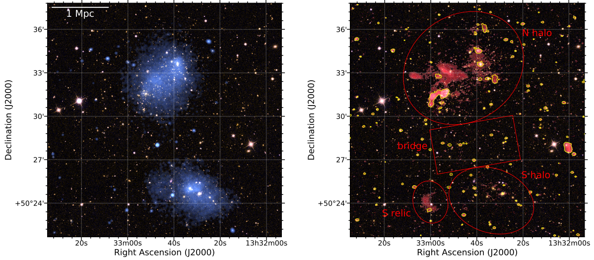
Figure 1. Composite images of A1758 obtained from the superposition of an optical SDSS g,r,i mosaic with Chandra (blue) and with a LOFAR image at 144 MHz with a resolution of 7.6'' \times 5.4'' (red) and a rms noise of 60 \mu\text{Jy beam}^{-1} . Yellow and red regions indicate the mask used to subtract discrete sources and the regions adopted to measure the flux densities in the low-resolution images, respectively.
