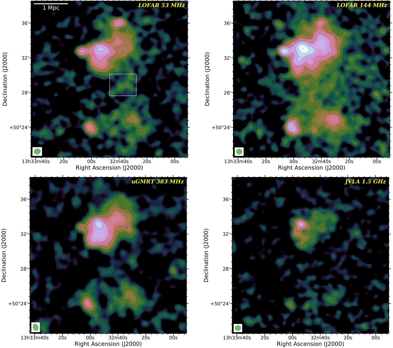
Figure 2. Radio images from 53 MHz to 1.5 GHz of A1758 with discrete sources subtracted. The color scale has a logarithmic stretch from 0.5 to 200\sigma . Contours are drawn from 3\sigma and are spaced by a factor of 2, where \sigma_{53\text{ MHz}} = 1.6\text{ mJy beam}^{-1} , \sigma_{144\text{ MHz}} = 160\text{ }\mu\text{Jy beam}^{-1} , \sigma_{383\text{ MHz}} = 170\text{ }\mu\text{Jy beam}^{-1} , \sigma_{1.5\text{ GHz}} = 80\text{ }\mu\text{Jy beam}^{-1} . Images were obtained by applying a Gaussian uv -taper of 35'' ; restoring beams are shown in the bottom left corners. The white box denotes the region where we measured a spectral index of \alpha = 1.65 \pm 0.27 between 53 and 144 MHz.
