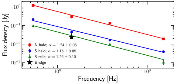
Figure 3. Integrated spectra of the diffuse radio sources.
