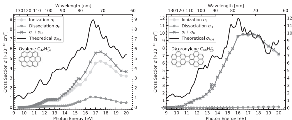
Figure 1. Experimentally determined cross sections for ionization, \sigma_I , and dissociation, \sigma_D , compared to the theoretically computed photoabsorption cross sections, \sigma_{\text{Abs}} , for ovalene (left panel) and dicoronylene (right panel).
