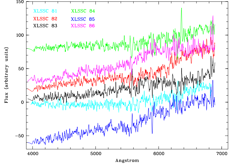
Fig. 3. Final reduced spectra of the BCG for all the clusters discussed here. Spectra have been shifted by arbitrary units to facilitate the viewing.
