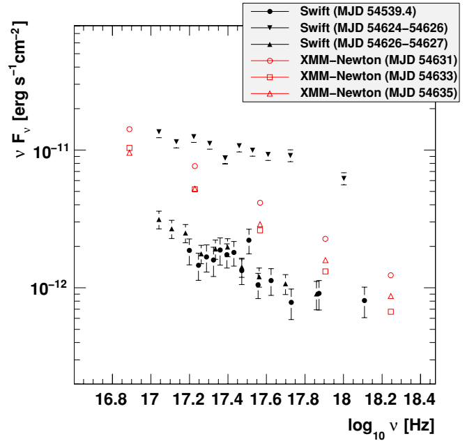
Figure 4. SED for five different X-ray measurements with Swift XRT and XMM-Newton EPIC for 2008 June 7–18 and the Swift XRT measurements in 2008 March (MJD 54539.4).
