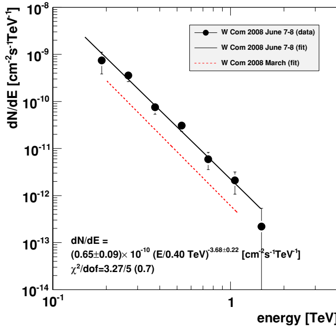
Figure 3. Differential VHE photon spectrum for W Com for MJD 54624.16 to 54625.24 (2008 June 7–8). The markers indicate measured data points and the continuous line a fit assuming a power-law distribution. Error bars show statistical errors only. For comparison, the photon spectrum of W Com derived from VERITAS measurements in 2008 March (Acciari et al. 2008b) is indicated by a dashed line.
