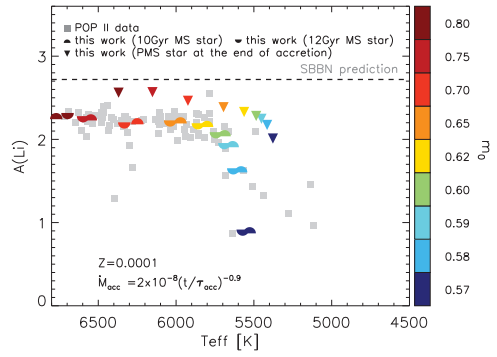
Figure 2. Our results in comparison with the lithium abundance measurements in Pop II stars. The grey filled squares are Pop II data from Molaro et al. (2012). Our predictions are shown for stars at the end of the late accretion phase (filled triangles), and on the main sequence at 10 Gyr (filled upper circle) and 12 Gyr (filled lower circle). Symbols are color-coded according to the initial stellar mass (legend on the right). The black dashed line marks the primordial Li abundance according to the SBBN.
