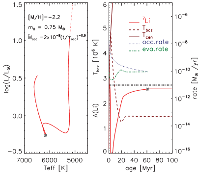
Figure 1. PMS evolution for a m_0 = 0.75 M_{\odot} , [M/H] = -2.2 star. Left panel: H-R diagram of the evolutionary track. The solid line starts when deuterium burning ends. The asterisk marks the end of the residual accretion. Right panel: Li evolution starting from A(\text{Li}) = 2.72 (horizontal line). The temperatures at the center ( T_{\text{cen}} , dark red dot dot dashed line) and at the base of the convection zone ( T_{\text{bcz}} , dark red dashed line) are also shown. The accretion rate is the dark blue dotted line while the EUV photo-evaporation is the dark green dot dashed line.
