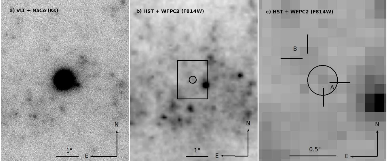
Figure 12. (a) The post-explosion image taken with VLT+NaCo 15 days after the explosion. (b) A pre-explosion image taken by HST/WFPC2 with the filter F814W. The scale and orientation of the images (a) and (b) are the same. The circle on (b) shows the position of the SN with 1\sigma uncertainty. The area marked with a square is enlarged in (c). The circle in (c) also shows the position of the progenitor, while A and B marks the sources detected with DOLPHOT (see text and Table 6).
