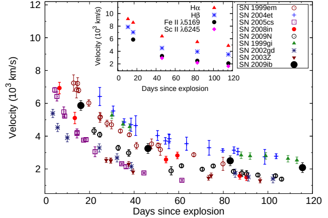
Figure 7. Comparison of the expansion velocities of SN 2009ib measured from the Fe II \lambda 5169 to those of the normal SNe II-P 1999em, 1999gi and 2004et, the subluminal SNe 2002gd, 2005cs, 2003Z and the intermediate luminosity SNe 2008in and 2009N. The insert shows Doppler-velocities from the absorption minima of H \alpha , H \beta , Fe II \lambda 5169 and Sc II \lambda 6245 lines of SN 2009ib.
