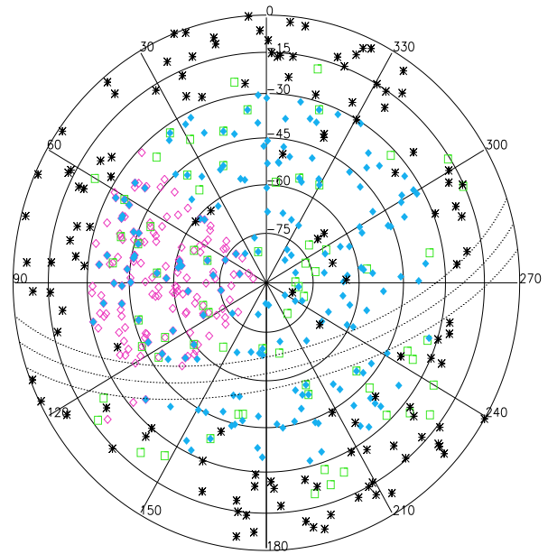
Figure 1. Polar projection of the southern sky, showing the distribution of the PACO samples (RA = 0 h is at the top and the RA increases counter-clockwise). The dotted lines indicate the Galactic plane and bound the area with Galactic latitude |b| < 5^\circ . Sources in these regions were excluded from the PACO samples. The faint PACO sample (open pink diamonds) occupies the area with 3^{\text{h}} < \text{RA} < 9^{\text{h}} . The bright PACO sample (filled blue diamonds) covers the whole area at \delta < -30^\circ . The spectrally selected sample (green squares), the blazars and the AT calibrator sources (black asterisks) are spread over the whole southern sky.
