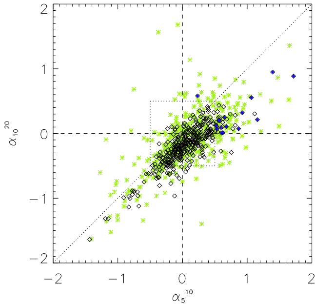
Figure 6. Colour-colour plot comparing the ~5–10 GHz and ~10–20-GHz spectral indices for the PACO best epoch data (black diamonds) and the AT20G data (green asterisks). Filled blue diamonds represent the objects that remained in the inverted-self-absorbed region of the plot at both observing epochs and hence are candidate to be GPS sources.
