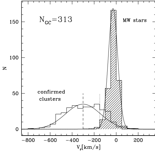
Fig. 5. Velocity distribution of confirmed M 31 clusters. The adopted systemic velocity of M 31 is marked by a dashed segment; the dotted segment marks the radial velocity threshold beyond which the contamination by foreground stars may become a serious issue. A Gauss curve with mean \mu = -301.0 \text{ km s}^{-1} and standard deviation \sigma = 160.0 \text{ km s}^{-1} is also superposed. The dashed histogram is the distribution of Galactic stars as predicted by the Besançon model (Robin et al. 2003), under the assumptions described in Sect. 4. A Gauss curve with mean \mu = -29.0 \text{ km s}^{-1} and standard deviation \sigma = 42.6 \text{ km s}^{-1} is also superposed.
