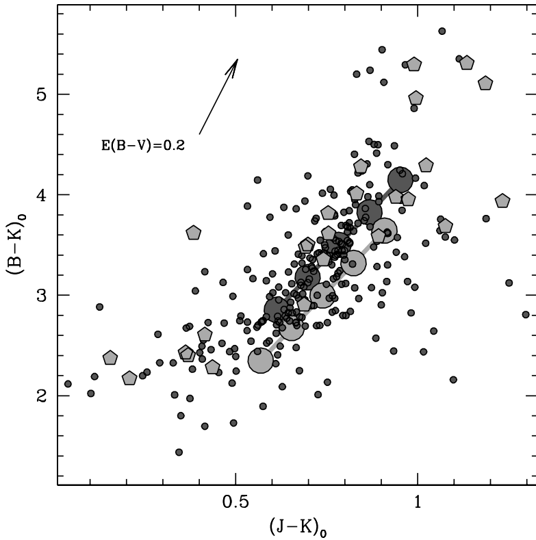
Fig. 11. Distribution of confirmed M 31 clusters in the reddening-corrected J - K vs. B - K plane. E(B - V) = 0.11 is assumed for all M 31 clusters. Small filled circles are previously confirmed clusters, pentagons are the newly confirmed clusters studied in the present paper. SSP model sequences by Buzzoni (1989), for fixed ages (i.e. 15 Gyr for the upper sequence and 2 Gyr for the lower sequence) and varying metallicity (from [Fe/H] = -2 to a solar value, at equal steps of 0.5 dex, see large solid dots in the sense of increasing J - K color along the sequences) are superposed. A Salpeter IMF slope and a red horizontal branch morphology is assumed in the models.
