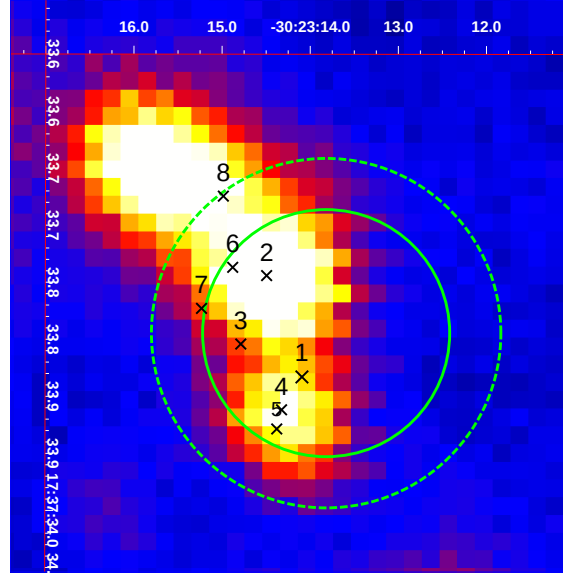
Figure 6. UKIDSS infrared map (K band) of the sky region around IGR J17375–3022, superimposed on the Swift /XRT error circles at 90% and 99% confidence level. Sources numbered from 1 to 8 are listed in Table 2
