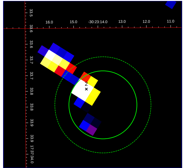
Figure 7. VVV infrared map (K band) of the sky region around IGR J17375–3022, superimposed on the Swift /XRT error circles at 90% and 99% confidence level
