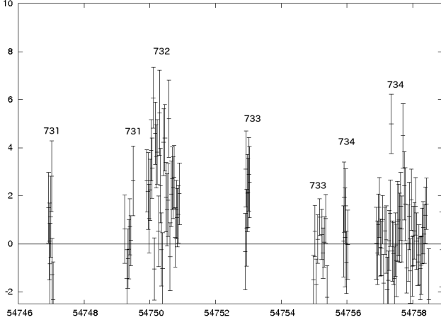
Figure 4. IBIS/ISGRI light curve (18–60 keV) at ScW level ( \sim 2,000 s bin time) of IGR J17375–3022 covering the period from revolution 731 to 734
