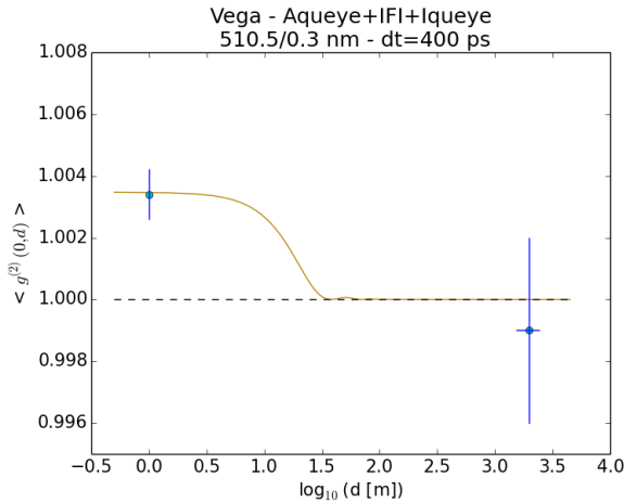
Figure 5. Spatial correlation \langle g^{(2)}(0, d) \rangle for the Aqueye+IFI+Iqueye 2019 observations of Vega. The yellow solid line represents the theoretical g^{(2)} for a uniform brightness disc of 3.3 mas (angular size of Vega; Ciardi et al. 2001; Monnier et al. 2012).
