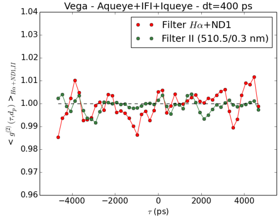
Figure 4. Temporal correlation on a \sim km baseline \langle g^{(2)}(\tau, d_p) \rangle_{H\alpha+ND1, II} for all the Aqueye+IFI+Iqueye Nov 2019 observations of Vega reported in Table 3 and for the two adopted combinations of filters, H\alpha +ND1 and II. The time bin is dt = 400 ps. Data is corrected for the light travel time delay between telescopes. The projected baseline d_p varied in the range 1535-2418 m.
