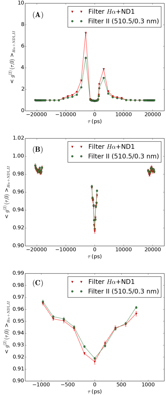
Figure 1. Temporal correlation at zero baseline for the Aqueye+ observations of Vega taken on Nov 28, 2019, calculated with a sampling time dt \approx 400 ps and for the two adopted combinations of filters, H\alpha+ND1 and II. The properties of the two sets of filters are reported in Table 3. Panel (A): measurements for delays \tau = [-20.5, 20.5] ns. Panel (B): measurements after removing the intervals \tau = [-18, -1] ns and \tau = [0.8, 18] ns. Panel (C): measurements for delays \tau = [-1, 0.8] ns.
