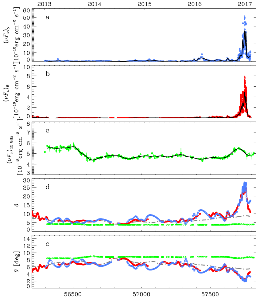
Figure 16. Light curves of CTA 102 in the \gamma -ray (a), optical (b), and 15 GHz radio (c) bands. The black curves indicate splines interpolations with variable time bin in the optical and \gamma -ray bands, and 30-d bins at 15 GHz; they represent the long-term trends. The Doppler factor \delta for the \gamma -ray (blue), the optical (red), and the radio (green) bands are plotted in panel (d), while (e) shows the corresponding viewing angles. In panel (d) and (e) the grey dot-dashed curve shows the trend obtained for the 230 GHz data according to Raiteri et al. (2017).
