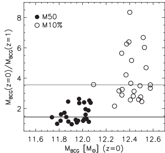
Figure 8. The individual BCG mass growth factor between z=1 and 0 as a function of BCG mass. Only the sample of BCGs extracted from main progenitor clusters is considered. Horizontal thick and thin lines stand for the median growth factor MGF, 1.4 and 3.6, for M50 and M10 per cent, respectively. The median growth factor for M30 is \sim 1.2 (not shown).
