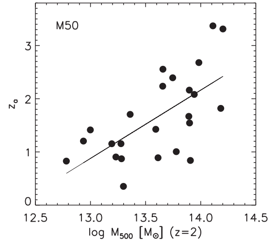
Figure 3. Assembly time z_a as a function of cluster mass at z=2 considering the main progenitor of the z = 0 BCG. The solid line is the best fit y = 1.28x - 15.82 . The Pearson correlation coefficient is 0.65.
