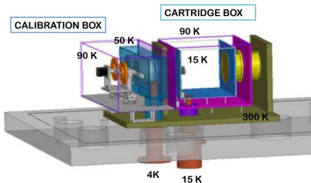
Figure 5. Left: sketch of the cartridge measurement concept inside the iALMA cryofacility. Right: cryogenic translator stage for the automatic movement of the cryogenic calibrator in front of the lens.
