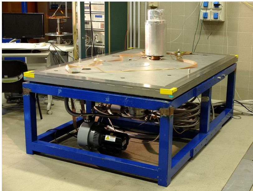
Figure 7. iALMA cryofacility.
