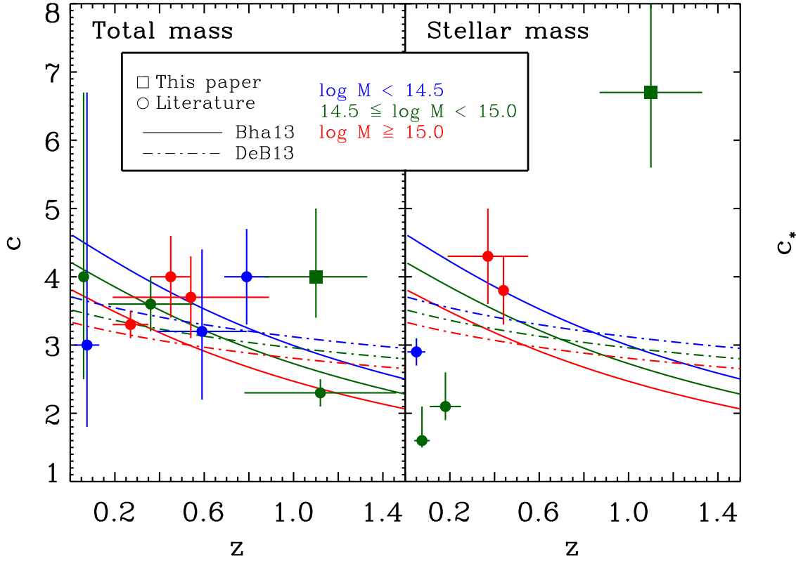
Fig. 7. Total and stellar mass concentration vs. redshift. The theoretical relations from Bhattacharya et al. (2013; solid lines) and from De Boni et al. (2013; dash-dotted lines) are shown for halos of masses \log M_{200}/M_{\odot} = 14.25, 14.75, 15.25 (blue, green, red curves, resp.). The data-points represent determinations of the total and stellar mass concentrations (left and right panel, resp.) from the literature and the present work (indicated by a square). The points are colored according to the average mass of the sample of clusters used for the determination of c : \log M_{200}/M_{\odot} < 14.5 (blue), 14.5 \leq \log M_{200}/M_{\odot} < 15.0 (green), \log M_{200}/M_{\odot} \geq 15.0 (red). The data references can be found in Table 3.
