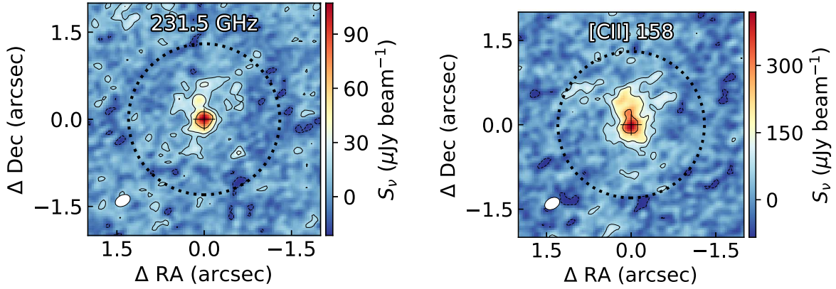
Figure 2. ALMA dust continuum (left) and [C II] (right) maps of J1342+0928. The 0''.28 \times 0''.20 ( 1.41 \text{ kpc} \times 0.99 \text{ kpc} ) beam size is shown at the bottom left of each panel while the cross indicates the peak of the dust continuum emission, which is consistent with the near-infrared position of the quasar. The solid (dashed) lines represent the +( - )2, 4, 8 \times \sigma contours with \sigma = 7.7 \mu\text{Jy beam}^{-1} for the continuum flux density at 231 GHz (left panel) and \sigma = 35.0 \mu\text{Jy beam}^{-1} for the [C II] flux density (right panel). The black dotted circles mark the 1''.3 ( 6.5 \text{ kpc} ) radius aperture used to measure the total flux densities.
