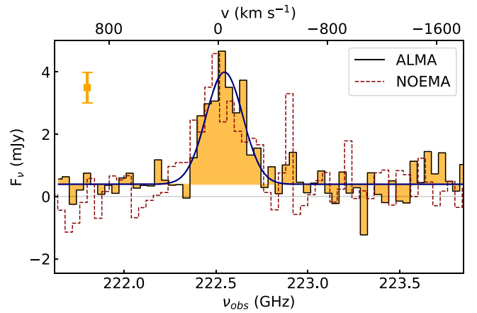
Figure 1. Spatially integrated [C II] spectrum of the quasar J1342+0928 within an aperture of 1''.3 radius. Standard deviation of the flux measurement is shown on the left. The blue line is a fit to the data consisting of a Gaussian on top of a flat continuum. The upper axis shows velocities centered at z = 7.5413 as reported in Venemans et al. (2017b), which is consistent with the value measured here from the ALMA data: z = 7.5400 \pm 0.0003 . Their NOEMA spectrum is also shown with a dashed line.
