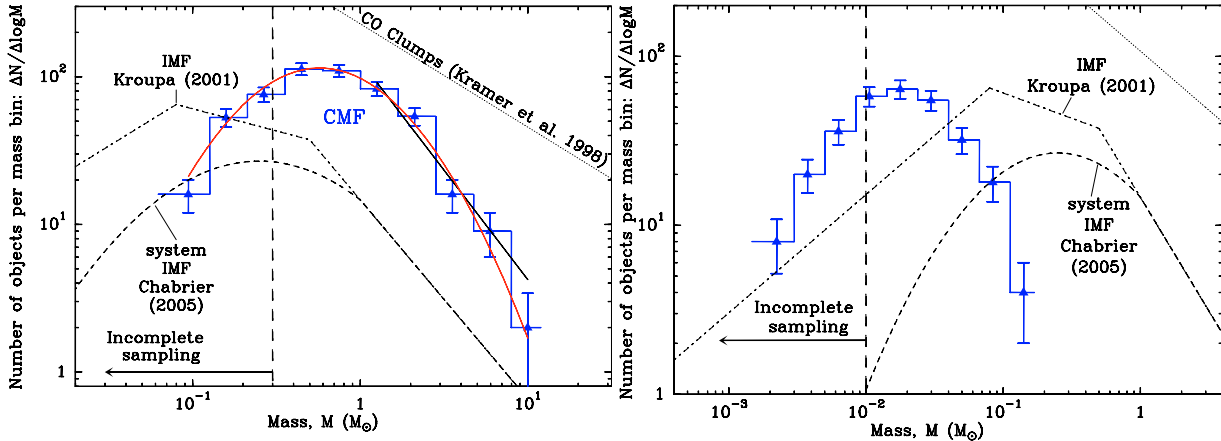
Fig. 2. Core mass functions (blue histograms with error bars) derived from our SPIRE/PACS observations of the Aquila ( left ) and Polaris ( right ) regions, which reveal of total of 541 candidate prestellar cores and 302 starless cores, respectively. A lognormal fit (red curve) and a power-law fit (black solid line) to the high-mass end of the Aquila CMF are superimposed in the left panel. The power-law fit has a slope of -1.5 \pm 0.2 (compared to a Salpeter slope of -1.35 in this dN/d\log M format), while the lognormal fit peaks at \sim 0.6 M_\odot and has a standard deviation of \sim 0.43 in \log_{10} M . The IMF of single stars (corrected for binaries – e.g., Kroupa 2001), the IMF of multiple systems (e.g., Chabrier 2005), and the typical mass spectrum of CO clumps (e.g., Kramer et al. 1998) are also shown for comparison. Note the remarkable similarity between the Aquila CMF and the stellar IMF, suggesting a \sim one-to-one correspondence between core mass and star/system mass with M_{\text{sys}} = \epsilon M_{\text{core}} and \epsilon \approx 0.4 in Aquila.
