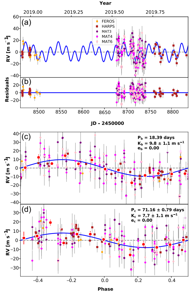
Figure 13. (a) Best-fitting two-planet Keplerian orbital model for TOI-257. The maximum likelihood model(s) is plotted in blue. We add in quadrature the radial velocity jitter terms listed in Table 4 with the measurement uncertainties for all radial velocities to determine individual error bars. (b) Residuals to the best-fitting 2-planet model. (c) Same, but radial velocities phase-folded to the period of planet b. (d) Same, but radial velocities phase-folded to the period of a possible planet c. Red circles (if present) are the individual velocities binned in 0.08 units of orbital phase.
