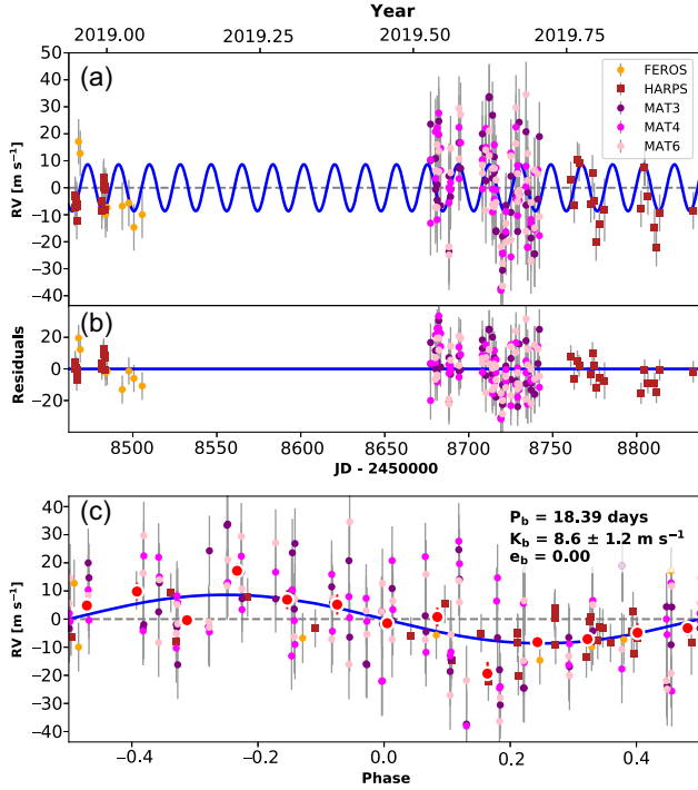
Figure 12. (a) Best-fitting one-planet Keplerian orbital model for TOI-257. The maximum likelihood model is plotted in blue. We add in quadrature the radial velocity jitter terms listed in Table 4 with the measurement uncertainties for all radial velocities to determine individual error bars. (b) Residuals to the best-fitting one-planet model. (c) Radial velocities phase-folded to the period of planet b. Red circles are the individual velocities binned in 0.08 units of orbital phase.
