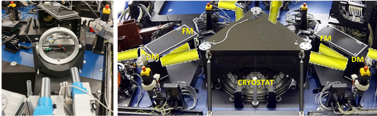
Fig 7. Left: the two ACT's facing the reference mirror. Right: FM and DM parallel to each other
