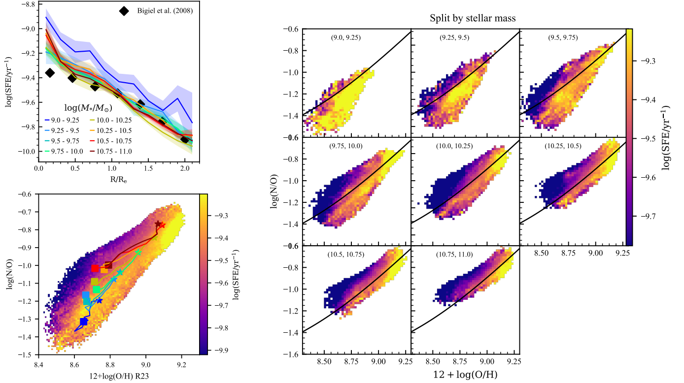
Figure 4. ( Top left ) The radial distribution of star formation efficiencies estimated from the MaNGA data. These are consistent with the Bigiel et al. (2008) estimates shown by the black diamonds. ( Lower left ) The distribution of \log(\text{N}/\text{O}) and 12 + \log(\text{O}/\text{H}) , with colours corresponding to the mean estimated star formation efficiency for spaxels falling in each cell in the image. At fixed oxygen abundance, regions of galaxies with higher N/O exhibit systematically lower SFE. We have plotted the median radial dependence for galaxies in the stellar mass range indicated by the colour of the line. ( Right ) We show distribution of N/O, O/H and the SFE, splitting the sample into bins of total galaxy stellar mass indicated at the top of each panel. The trend seen in the full sample is reflected in each mass bin, though each interval of stellar mass covers different parts of the N/O vs O/H plane. The \xi = 0 line is marked in black.
