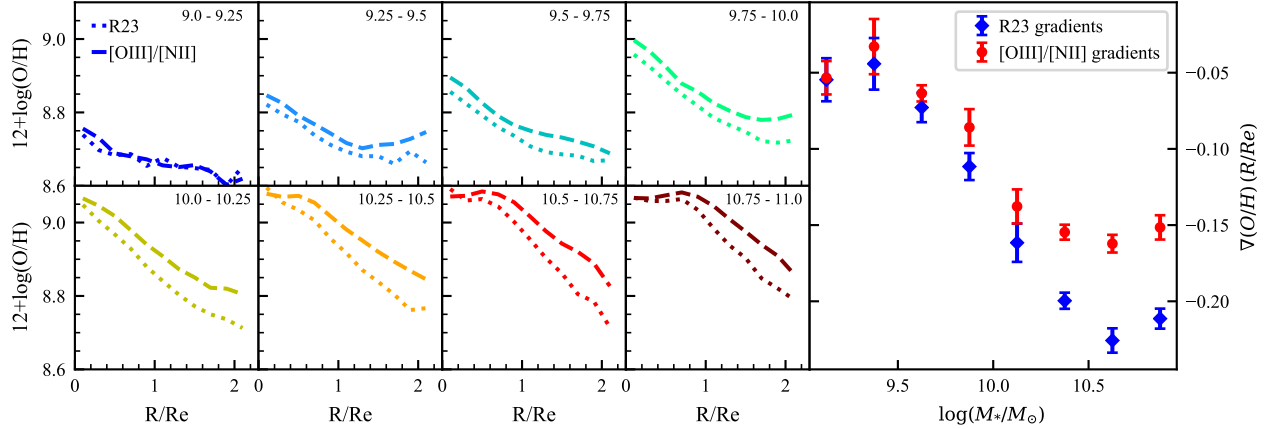
Figure 3. Discrepancies in the inferred radial profiles of oxygen for the two different abundance indicators. The small panels show the radial profiles of 12 + \log(\text{O}/\text{H}) as derived by R23 (dotted) and [\text{OIII}]/[\text{NII}] (dashed). Profiles are shown for galaxies within the range of stellar masses indicated at the top right of each panel. While [\text{OIII}]/[\text{NII}] gives slightly higher O/H, the gradients are also flatter. The gradients are shown as a function of stellar mass in the large panel on the right. The difference between the gradients yielded by the two indicators grows with stellar mass, culminating in a disagreement of approximately 40 per cent above \log(M_*/M_\odot) > 10.5 .
