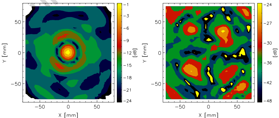
Fig. 10 Same as Fig. 9 for the three-coronae TP
