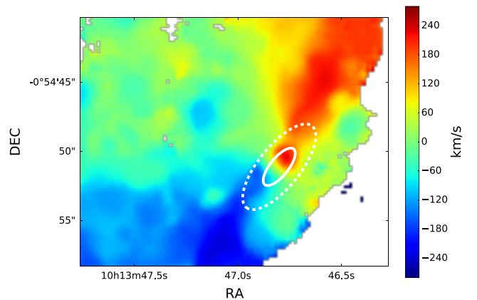
Figure 6. The radio continuum sources overlaid on H I velocity field. The solid and dotted white ellipses at the centre represent the estimated size of the continuum source based on the FIRST and GASP observations, respectively. The colour bar is velocity of H I gas in \text{km s}^{-1} . Evidently, there is a steep velocity gradient across the radio continuum source.
