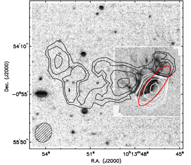
Figure 4. The JVLA H I column density contours are overlaid on MUSE H\alpha map: black contours are H I emission with contour levels at (0.25, 0.5, 1, 2) \times 10^{20} \text{ cm}^{-2} ; white contours represent H I absorption with contour levels at (-1, -2, -4, -8) \text{ mJy beam}^{-1} . Outside the extent of the MUSE pointing, the background is the INT B -band image. The red ellipse is the tracer of the stellar disc. The FWHM beam size of 20.7 \text{ arcsec} \times 15.6 \text{ arcsec} is in the bottom left of the plot.
