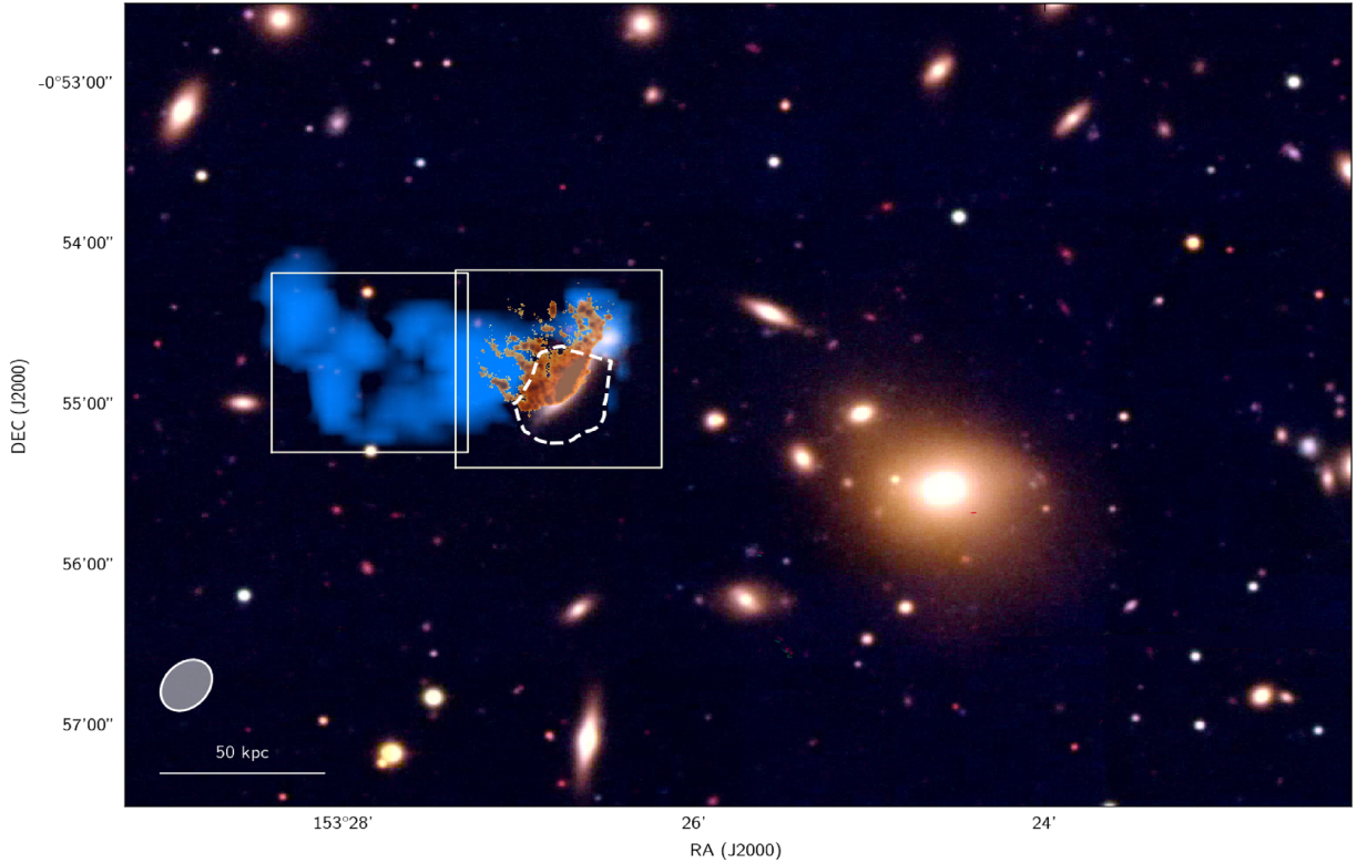
Figure 1. RGB image of central region of A957 from OmegaWINGS u - and WINGS B - and V -band images (Gullieuszik et al. 2017) overlaid with the total H\alpha emission (in orange) and total H\text{I} emission (in blue). The dotted line is the H\text{I} absorption contour ( -1 mJy). The white square boxes in right and left are the old and new MUSE pointings, respectively. The grey shaded ellipse in the bottom left corner is the JVL A beam size ( 20.7 arcsec \times 15.6 arcsec).
