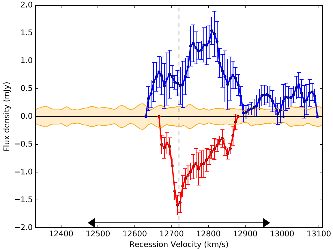
Figure 5. H I global profiles: blue and red profiles are emission and absorption profiles, respectively. The dotted in the middle is the systemic velocity ( 12\,720\text{ km s}^{-1} ) based on the stellar component at the centre of the galaxy. The horizontal line with arrows on either side is a representative of the width of global profile as expected from the Tully–Fisher (TF) relation. We have added a yellow band, showing the rms noise as a function of recession velocity. We have considered region of single beam size to calculate the rms as a function of recessional velocity.
