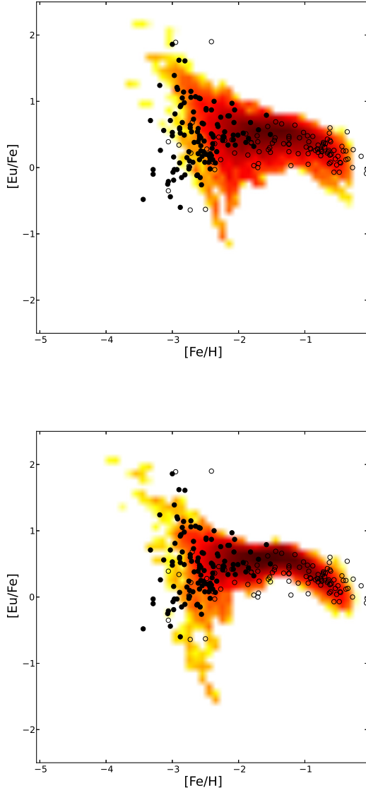
Fig. 3 Upper panel: the [\text{Eu}/\text{Fe}] vs. [\text{Fe}/\text{H}] relation predicted and observed in stars of the Milky Way halo. The model prescriptions for Eu production are the same as in the model of Figure 1 but the model allows for inhomogeneous mixing as described in Cescutti et al. (2015). Data are from Frebel (2010) (open and filled circles). Our model predictions are represented by the colored area. Lower panel: the model prescriptions for Eu production assumes a lower yield for Eu per merging event and 100 Myr fixed delay plus the contribution of magneto-rotationally driven SNe. Figure from Cescutti et al. (2015)
