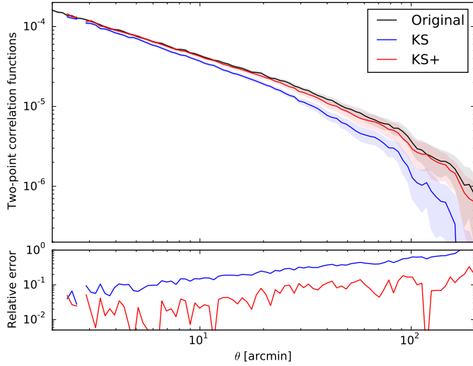
Fig. 13. Shape noise effects: mean shear two-point correlation function \xi_+ (black) and corresponding mean convergence two-point correlation function \xi_{\kappa_E} estimated from complete noisy shear fields. The convergence maps have been estimated using the KS method (blue) and using the KS+ method (red). The shaded area represents the uncertainties on the mean estimated on 1000 \text{ deg}^2 . Lower panel: relative two-point correlation error introduced by shape noise.
