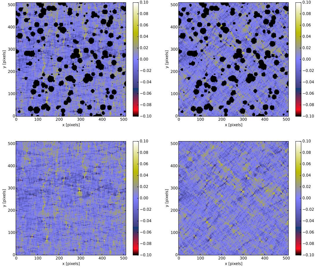
Fig. 1. Simulated shear maps with missing data covering a field of 5^\circ \times 5^\circ . Left panels : first component of the shear \gamma_1 , and right panels : second component of the shear \gamma_2 . Upper panels : incomplete shear maps, where the pixels with no galaxies are set to zero (displayed in black). Lower panels : result of the inpainting method that allows us to fill the gaps judiciously.
