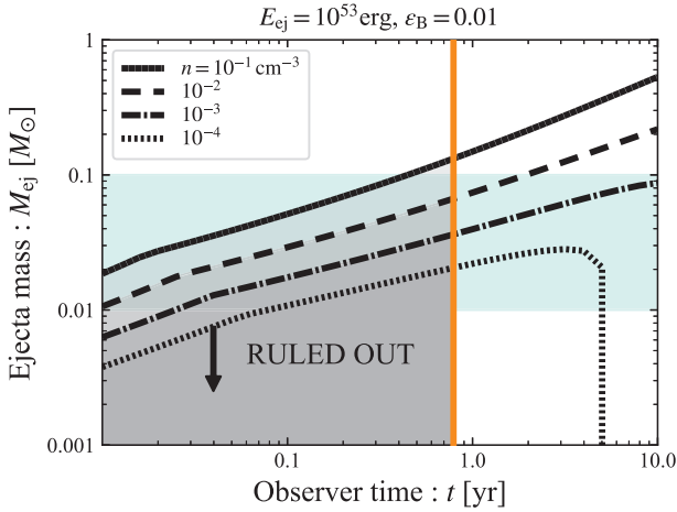
Figure 4. Ejecta mass ruled out by null detection F_v < 7.8 \mu\text{Jy} as a function of time. For a fixed density, only values above each curve are allowed by the data. The vertical orange line denotes the observation time in this work (288 d). The shaded region represents the relevant range of ejecta mass.
