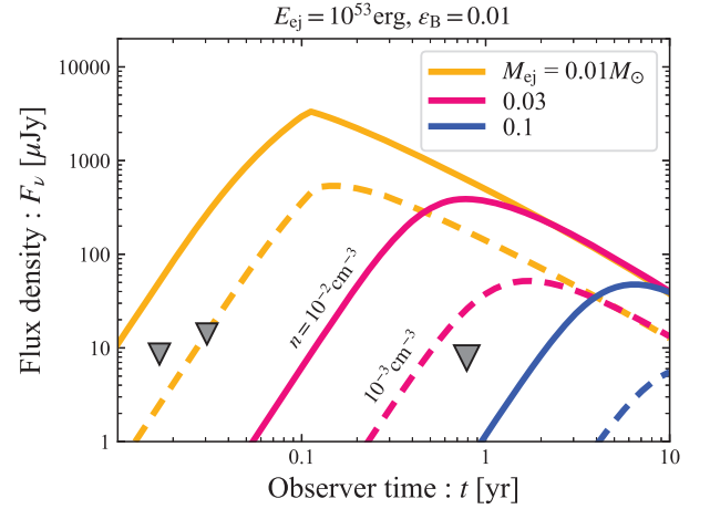
Figure 2. Light curves of GRB 200522A for various ejecta masses of M_{ej} = 0.01, 0.03 , and 0.1 M_\odot (the corresponding initial Lorentz factors \Gamma_{in} = 6.6, 2.9 , and 1.6 or \beta_{in} = 0.77 for the last case). Solid and dashed lines correspond to densities 10^{-2} and 10^{-3} \text{ cm}^{-3} , respectively. The other parameters are \epsilon_e = 0.1 , \epsilon_B = 0.01 , and p = 2.5 . Gray triangles show 3\sigma flux density upper limits from earlier observations by Fong et al. (2021), and our late-time monitoring.
