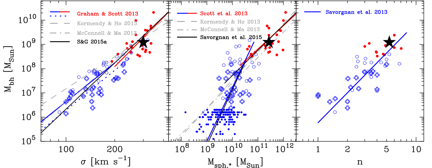
Figure 11. Left panel: M_{\text{bh}}-\sigma data and relations from Graham & Scott (2013): core-Sersic galaxies (red dots and red line); unbarred Sersic galaxies (blue circles and blue line); barred galaxies (blue crosses and blue dotted line). Middle panel: M_{\text{bh}}-M_{\text{sph},*} data and relations from Scott et al. (2013): core-Sersic galaxies (red line); barred and unbarred Sersic galaxies (blue line). The small blue dots denote AGN from Graham & Scott (2015) but were not used to derive the blue line. Right panel: M_{\text{bh}}-n data and relation from Savorgnan et al. (2013): barred and unbarred Sersic galaxies (blue line). The black star denotes NGC 1277. Note: Kormendy & Ho (2013) adjusted the central velocity dispersions to create reduced velocity dispersion estimates within R_e/2 ( \sigma_{R_e/2} ) to which their shallower M_{\text{bh}}-\sigma relation pertains. “S&G 2015a” refers to the relation for unbarred galaxies from Savorgnan & Graham (2015) while Savorgnan et al. (2015) refers to their relation for late-type galaxies, derived using the modified FITEXY routine from Tremaine et al. (2002) in a symmetrical manner.
