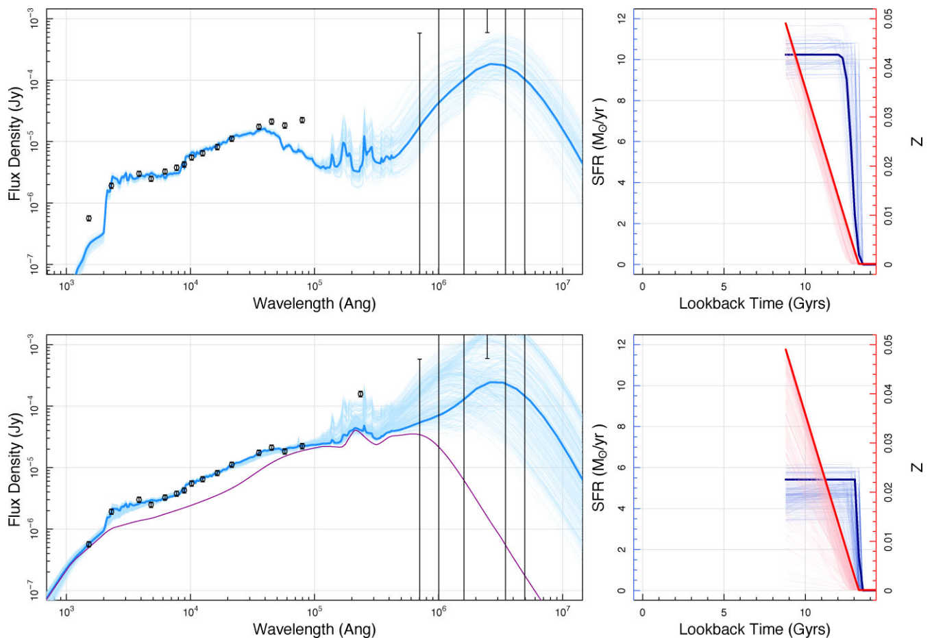
Figure 3. Here, we present example SED outputs as a function of observed wavelength for galaxy 101494591582430080 at z = 1.24 fit without and with an AGN component in the upper and lower panels, respectively. The MIPS24 data point is not shown in the upper panel as bands within the PAH features were removed from the fitting when an AGN component was not included (see Thorne et al. 2021). We show the contribution from the AGN component in the lower panel as the purple line. The left-hand panels show the input photometry (black circles and error bars), the best-fitting SED in blue and the SED generated from each step of the final MCMC chain in pale blue. The right-hand panels show the best-fitting SFH in blue and the posterior sampling in pale blue with the scaling given by the left axis. The metallicity history for each galaxy is also presented in the right-hand panel as the red line for the best-fitting solution and as the pink lines for sampling of the posterior. The scale of the metallicity history is shown on the right axis.
