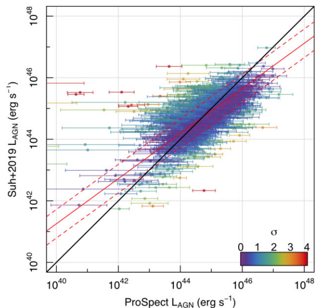
Figure 15. The bolometric AGN luminosity derived from PROSPECT compared to that derived in Suh et al. (2019). We show objects with a PROSPECT-derived f_{\text{AGN}} > 0.1 . The solid red line shows the best linear fit from HYPER-FIT and the dashed lines show the one standard deviation range. The points are coloured by their ‘sigma-tension’ from the linear fit and the black line denotes a one-to-one relation.
