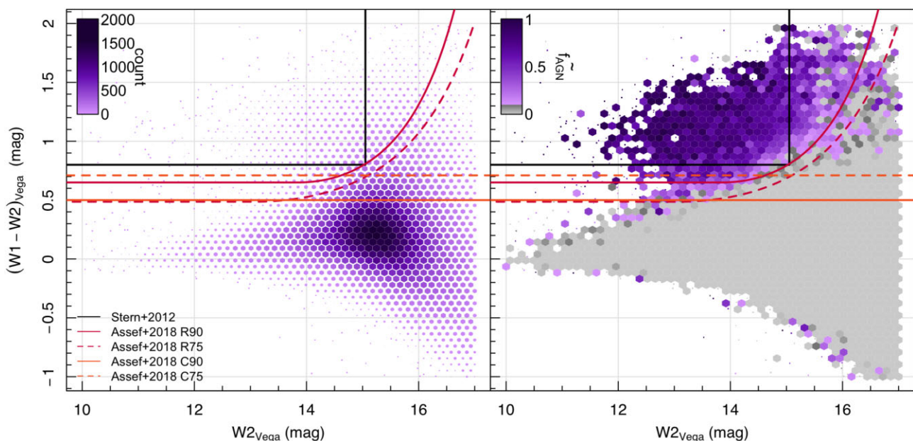
Figure 11. The left-hand panel shows the number distribution of the GAMA sample in WISE colour–magnitude space where both the colour and size of the hexagons represent the number of objects in each bin. The right-hand panel shows the WISE colour–magnitude coloured by median PROSPECT-derived f_{\text{AGN}} in each bin. Bins with a median f_{\text{AGN}} < 0.1 are shown in grey, and bins with increasing f_{\text{AGN}} > 0.1 are shown in darker shades of purple. We show the commonly used WISE colour selections from Stern et al. (2012) and Assef et al. (2018) in both panels. The Assef et al. (2018) relations are shown for the 75 (dashed) and 90 per cent (solid) completeness (orange) and reliability (red) cuts.
