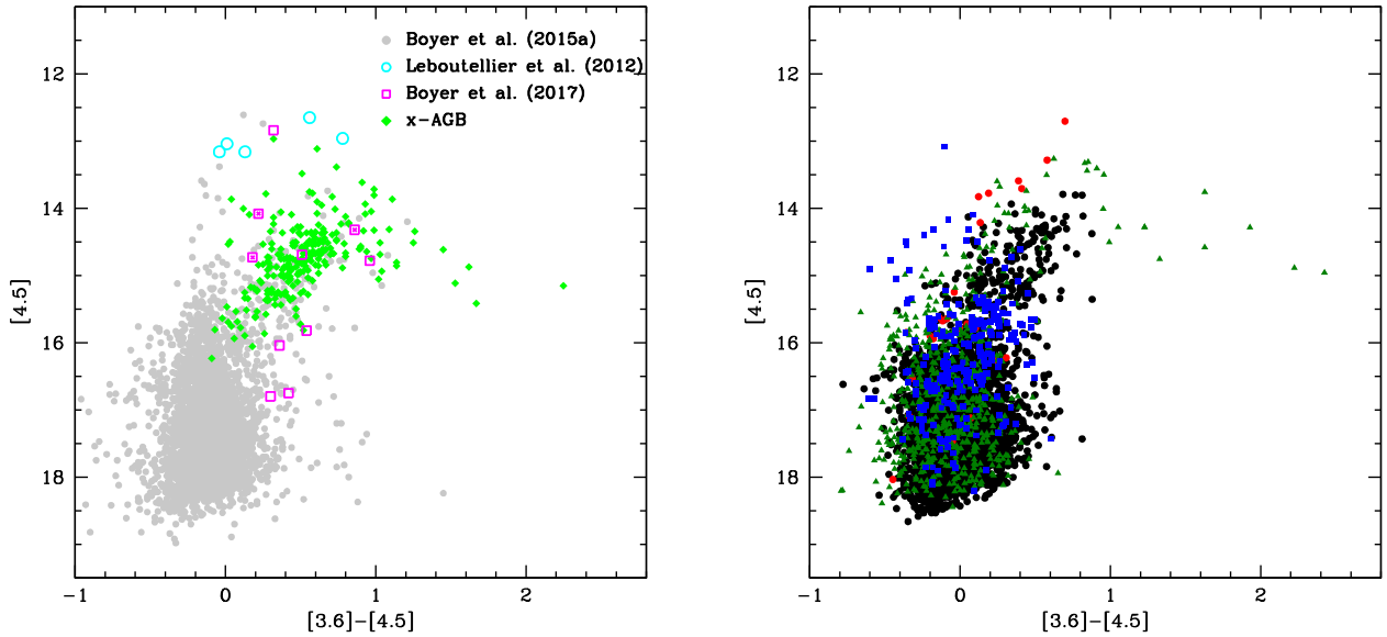
Figure 7. Left: The distribution on the colour–magnitude ( [3.6] - [4.5] , [4.5] ) plane of the IC10 stars from Boyer et al. (2015a), indicated with grey points. Cyan circles indicate the bright, O-rich stars by Leboutellier et al. (2012), whereas the obscured stars by Boyer et al. (2017), classified as O-rich, are indicated with magenta squares (crosses inside the square mean variable sources). The x-AGB stars by Boyer et al. (2015b) are represented with light green diamonds. Right: The results from synthetic modelling, with the same symbols used in Figs 4 and 5.
