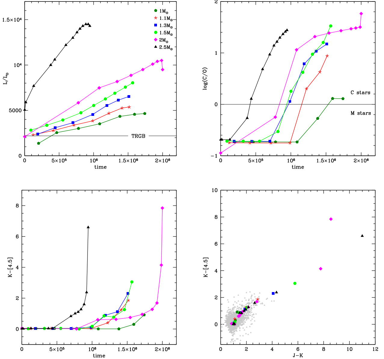
Figure 2. The evolution of the luminosity (top, left-hand panel) and of the C/O ratio (top, right-hand panel) of 1\text{--}2 M_{\odot} at Z = 10^{-3} and 2.5 M_{\odot} at Z \leq 2 \times 10^{-3} . The thin, horizontal lines mark the location of the TRGB and the boundary between M stars and carbon stars. The variation of the (K-[4.5]) colour is shown in the bottom, left-hand panel. We also show the excursions in the colour-colour ( J-K ) versus (K-[4.5]) plane, overimposed to the data of the IC10-evolved stellar population by Gerbrandt et al. (2015) and Boyer et al. (2015a). The adopted reddening is E(B - V) = 1.14 mag (see Section 5.2).
