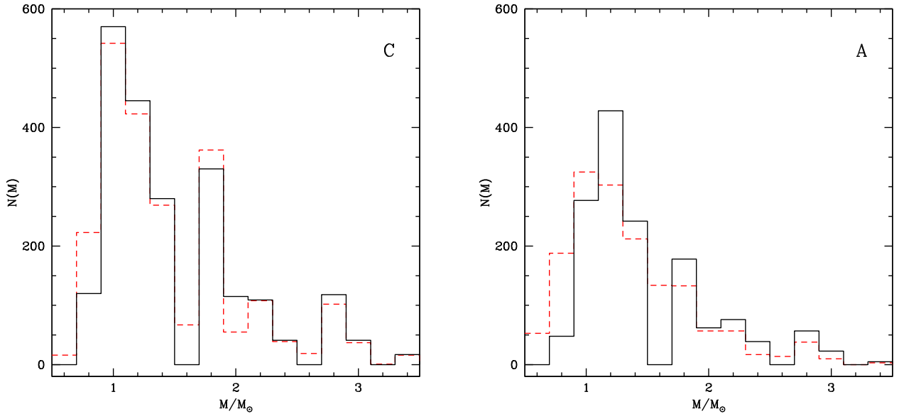
Figure 6. The progenitors mass distribution (black, solid lines) and the current mass (red, dashed) of the stars populating regions C (left-hand panel) and A (right-hand panel) in Fig. 5.
