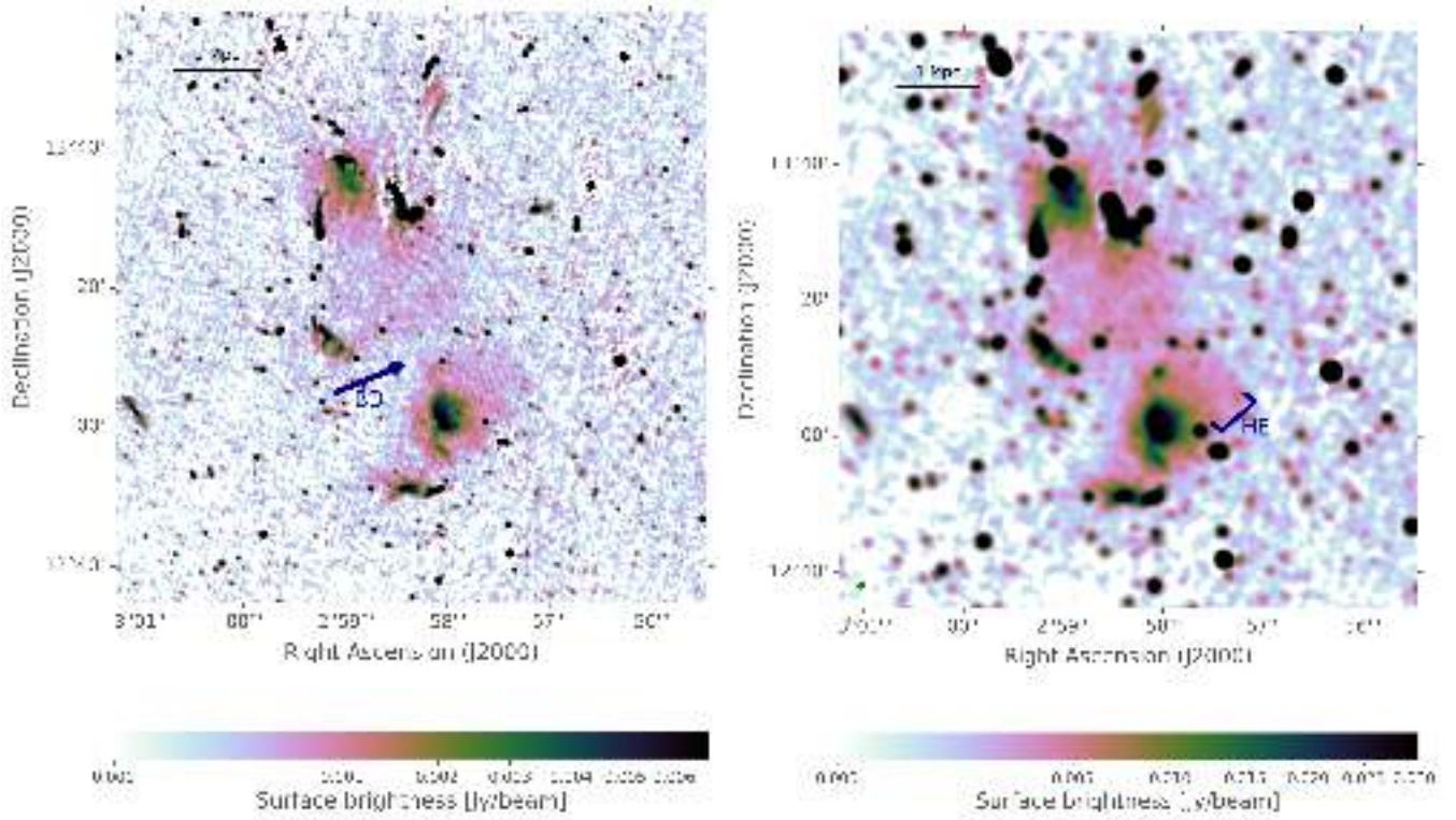
Fig. 5. Radio maps of the A399-401 system at lower resolutions. Left panel: resolution of 24.6'' \times 27.1'' with \sigma = 230 \mu\text{Jy beam}^{-1} . Right panel: resolution 72.8'' \times 75.9'' with \sigma = 809 \mu\text{Jy beam}^{-1} . The dark blue brightness depression (BD) and the halo extension (HE) are described in the text. The beam size in all images is given in the lower left corner , and the scale of 1 Mpc at z = 0.072 is given in the upper left corner . The square-root color scale of the images extends from 0 to 25\sigma .
